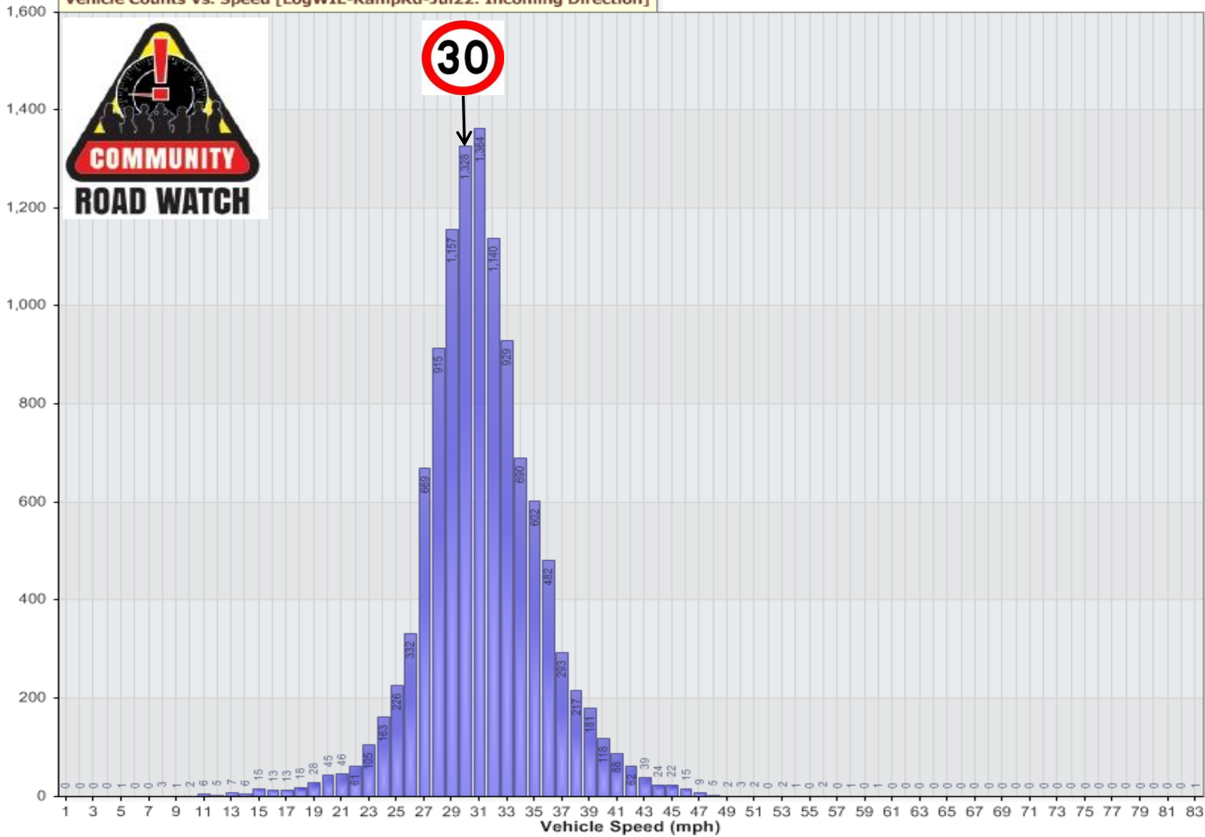
Vehicle Counts Vs. Speed [LogWIL-RampRd-Jul22: Incoming Direction]
