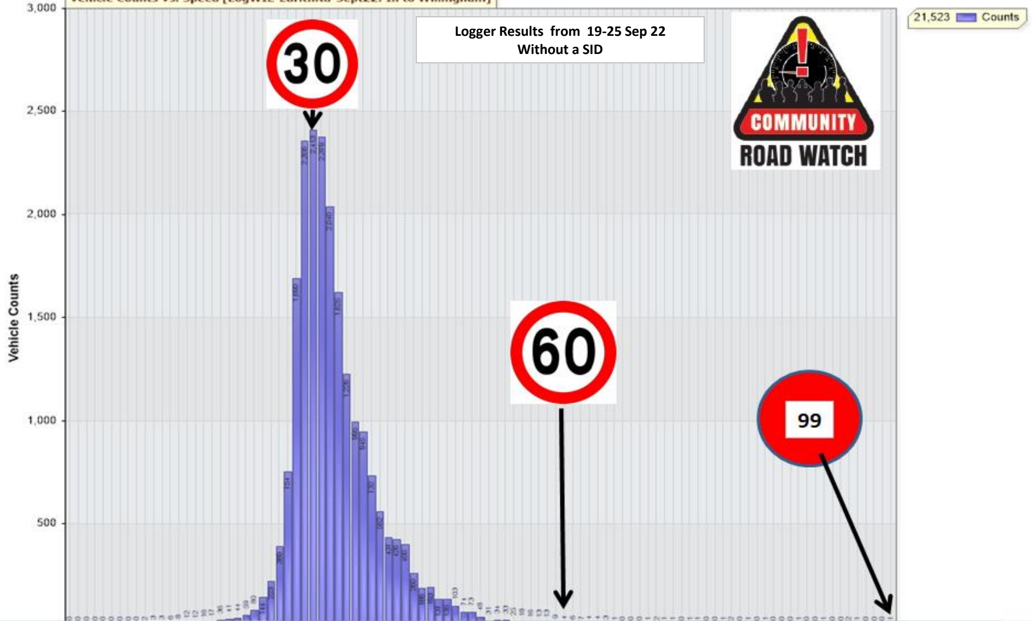
Vehicle Counts Vs. Speed [LogWIL-EarithRd-Sept22: In to Willingham]
