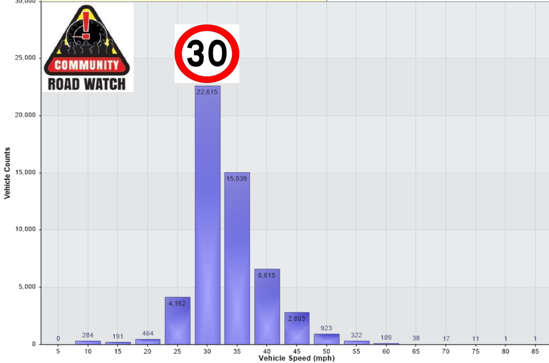
Vehicle Counts Vs. Speed [WIL-EarithRd-SID-IBAt76-Oct22: Incoming Direction]
