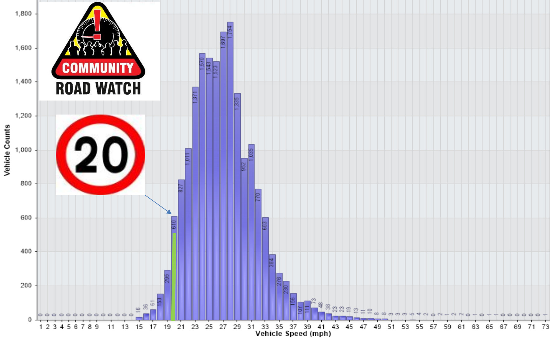
Vehicle Counts Vs. Speed [LogWil20-StnRd-FIB-Opp Camera-Sep25: Outgoing Direction]
