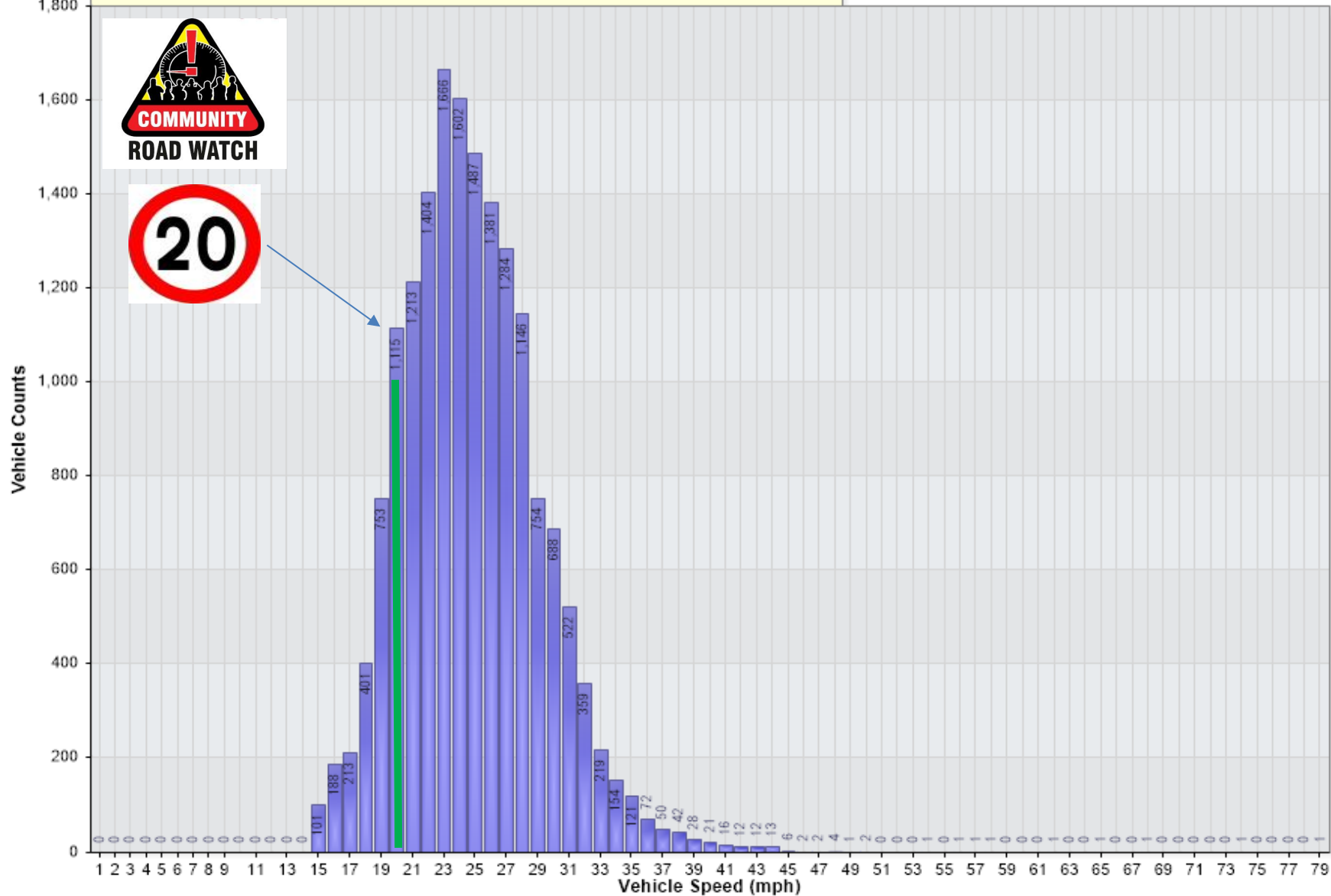
Vehicle Counts Vs. Speed [LogWil20-StnRd-FIB-Opp Camera-Sep25: Incoming Direction]
