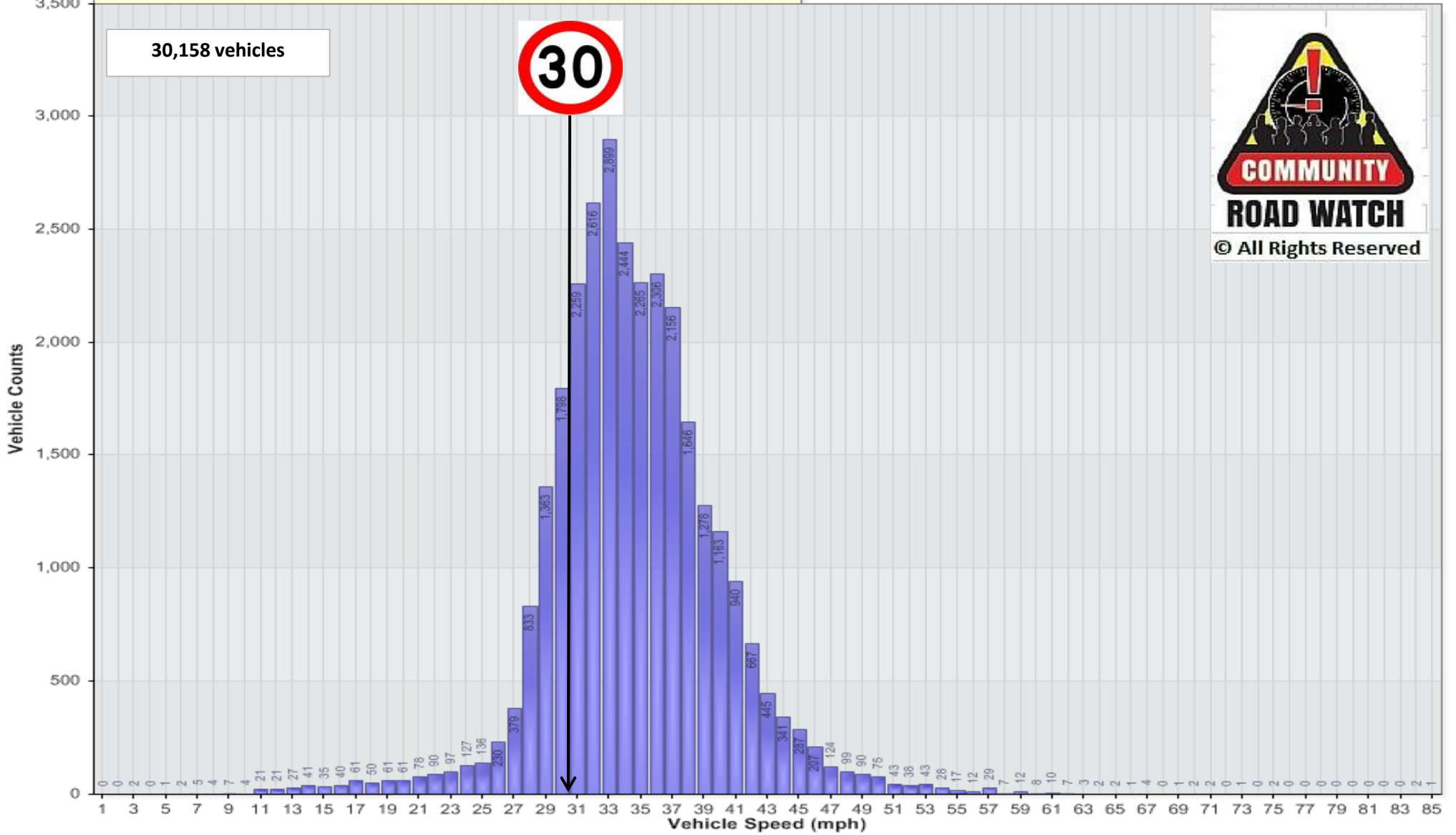
Vehicle Counts Vs. Speed [logWIL-StnRd30-SCS: Imported Data [Outgoing]]
