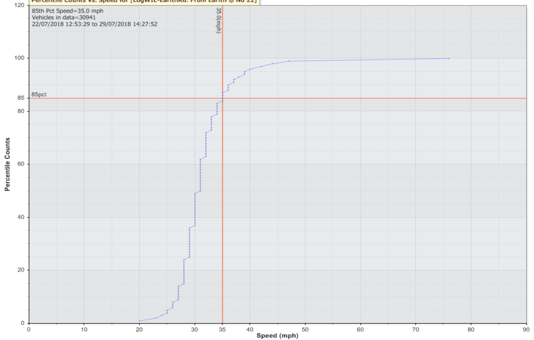
Percentile Counts Vs. Speed for [LogWIL-EarirthRd: From Earith @ No 22]
