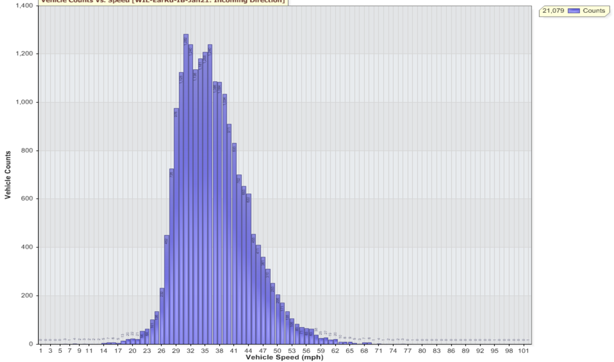
Vehicle Counts Vs. Speed [WIL-EarRd-IB-Jan21: Incoming Direction]
