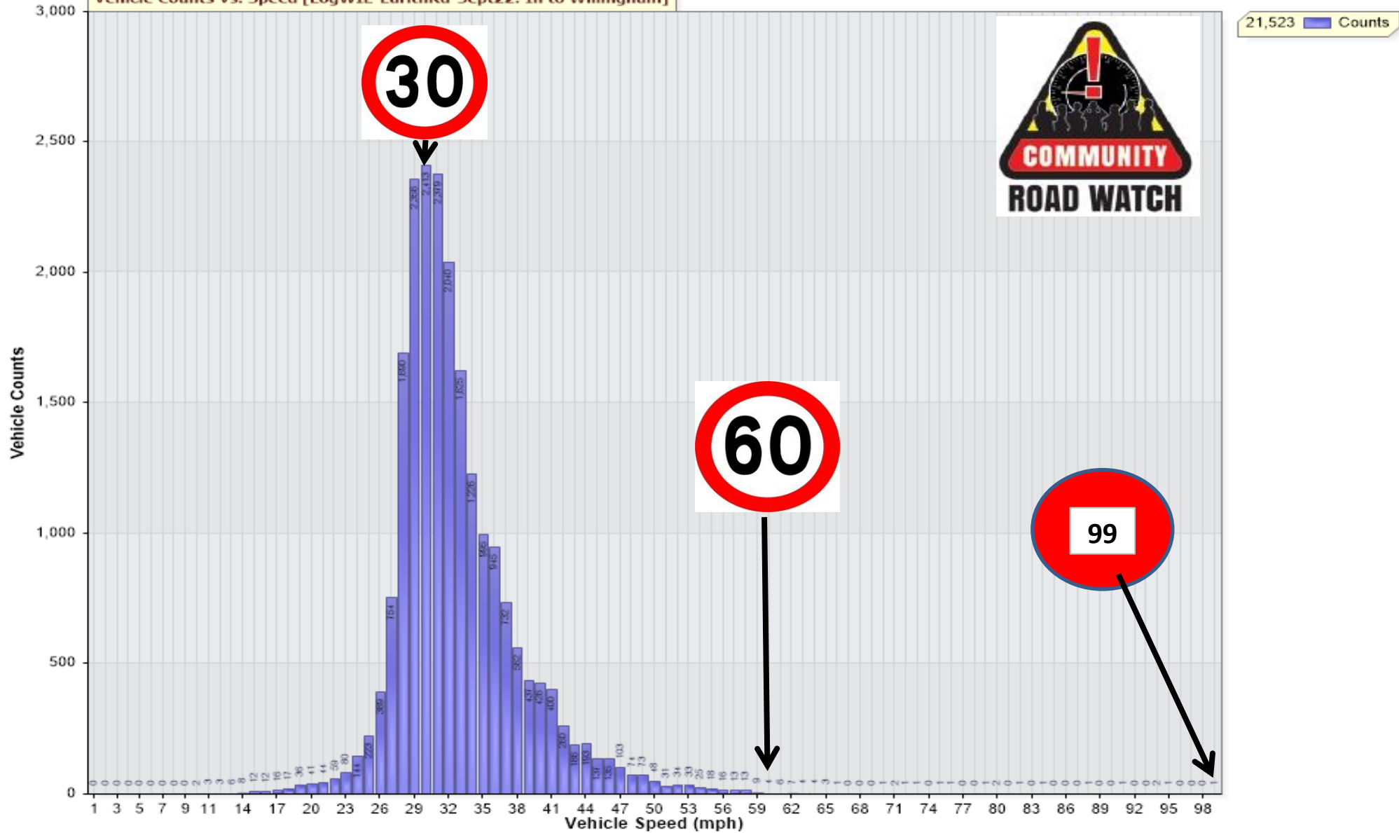
Vehicle Counts Vs. Speed [LogWIL-EarirthRd-Sept22: In to Willingham]
