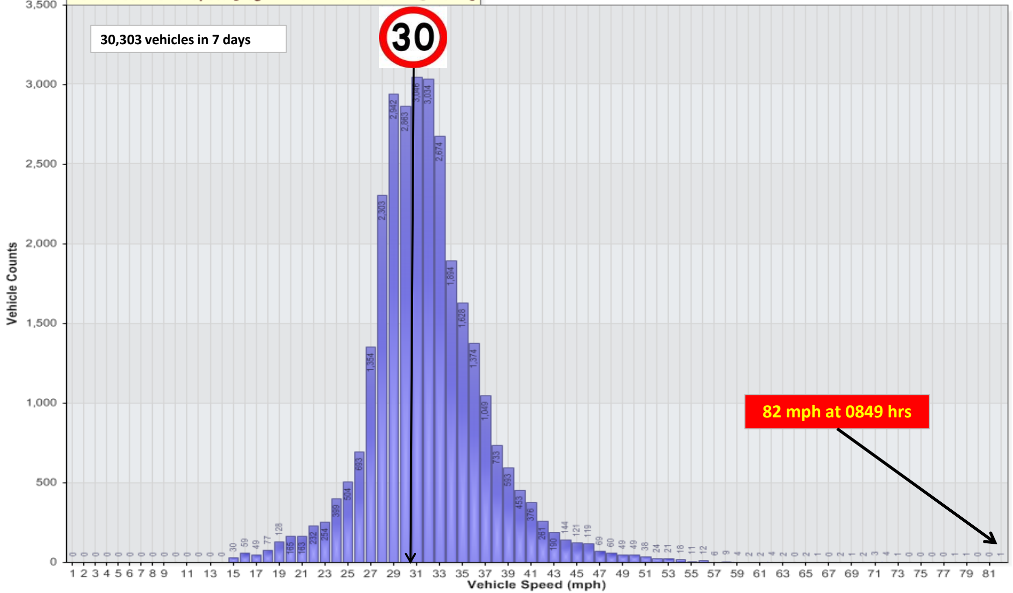
Vehicle Counts Vs. Speed [LogWIL-EarirthRd: To Earith @ No 22]
