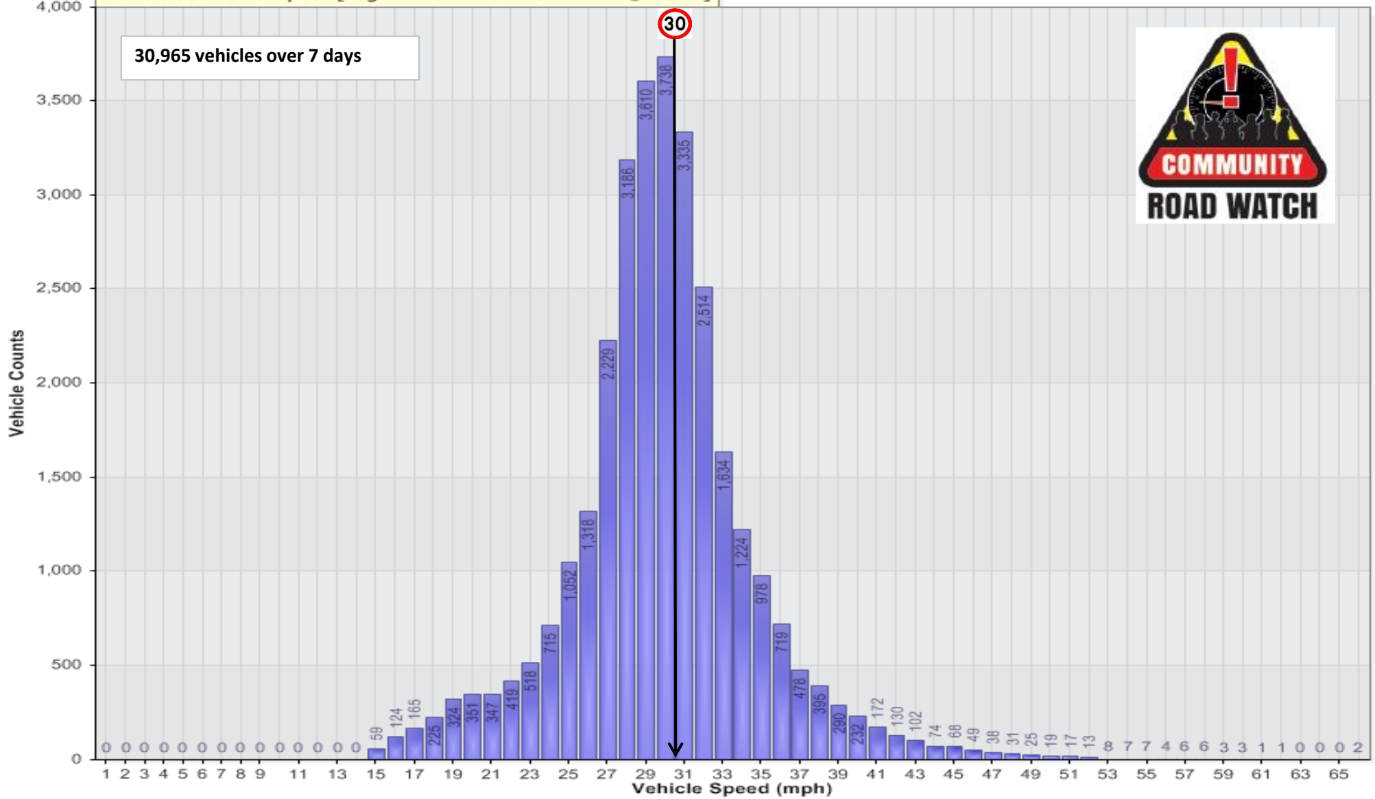
Vehicle Counts Vs. Speed [LogWIL-EarithRd: From Earith @ No 22]
