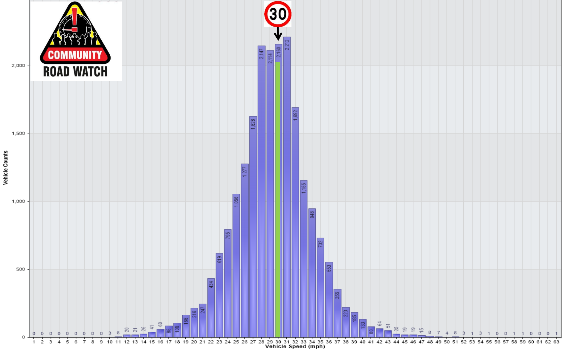
Vehicle Counts Vs. Speed [LogWIL-EarRd-AtPeglar-FOB-Apr25: Out to Earith]
