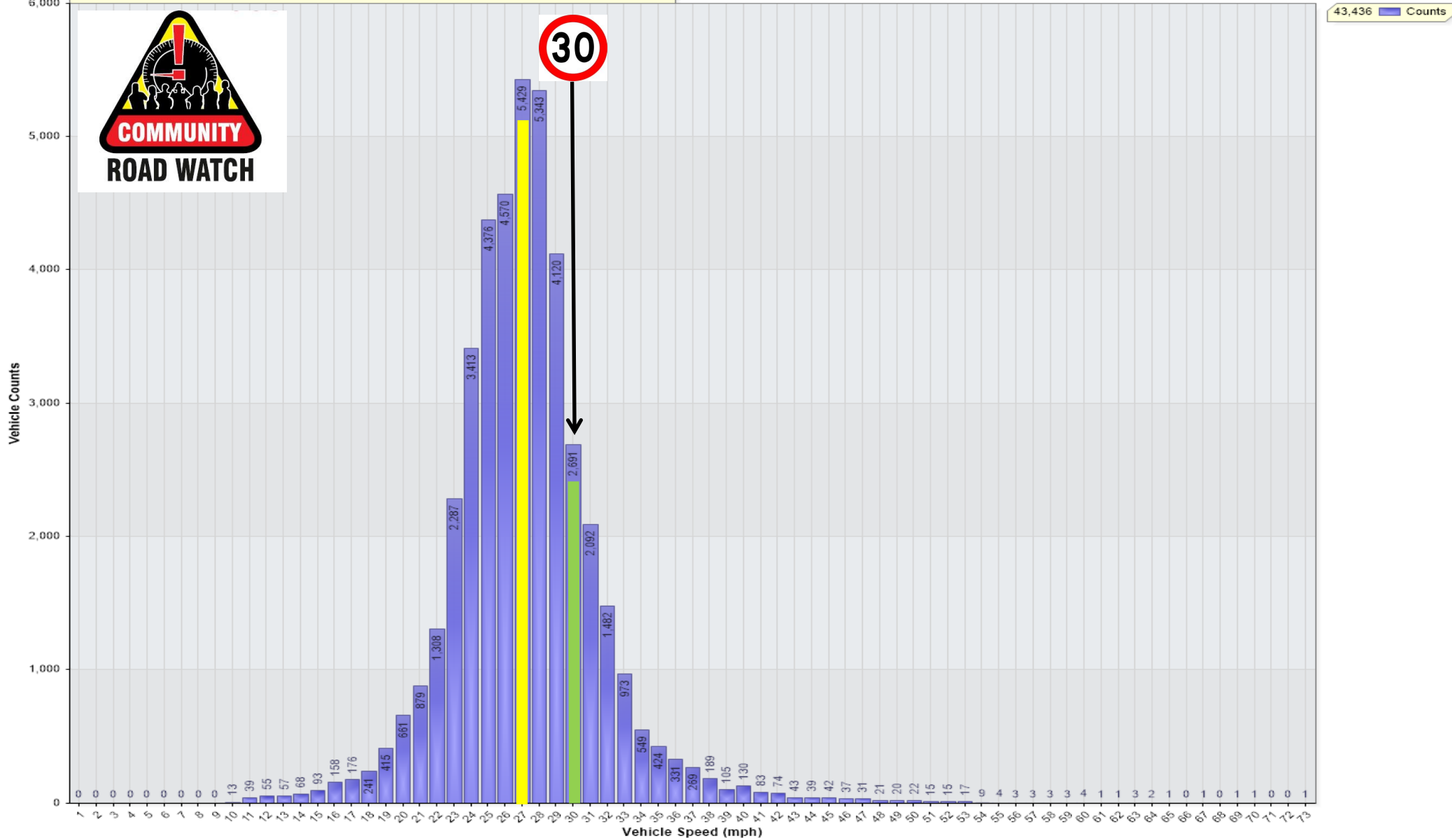
Vehicle Counts Vs. Speed [LogWIL-EarRd-AtPeglar-FOB-May25-Post20: Inbound from Earith]
