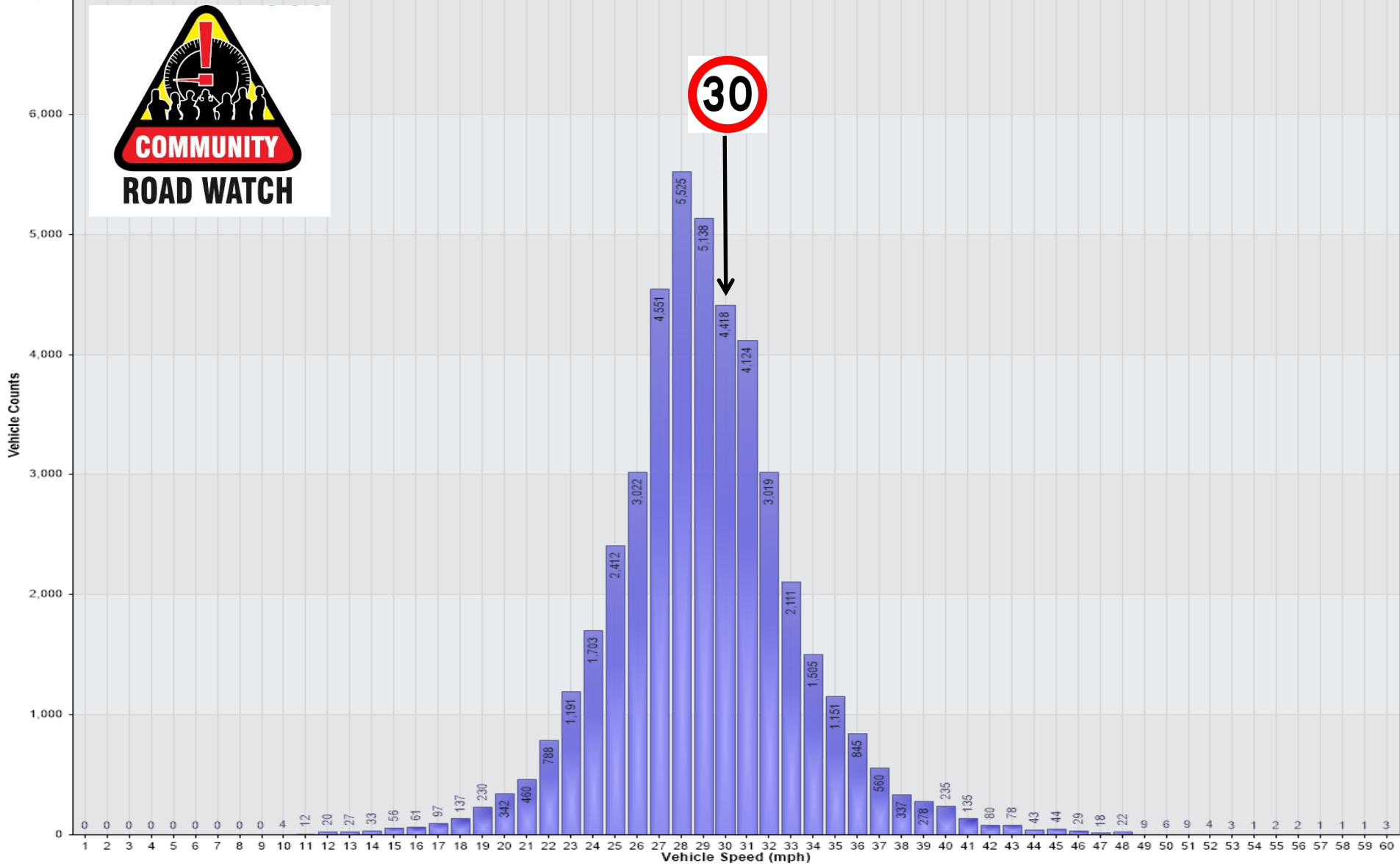
Vehicle Counts Vs. Speed [LogWIL-EarRd-AtPeglar-FOB-May25-Post20: Outbound to Earith]
