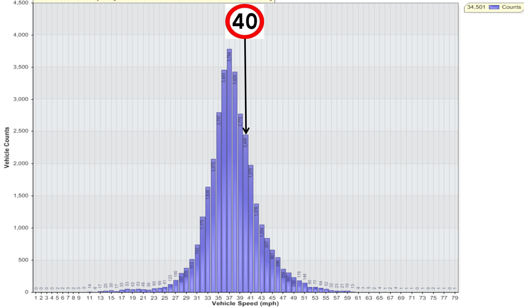
Vehicle Counts Vs. Speed [WBN-StrethamR?-Dec20: Inbound From Stretham]
