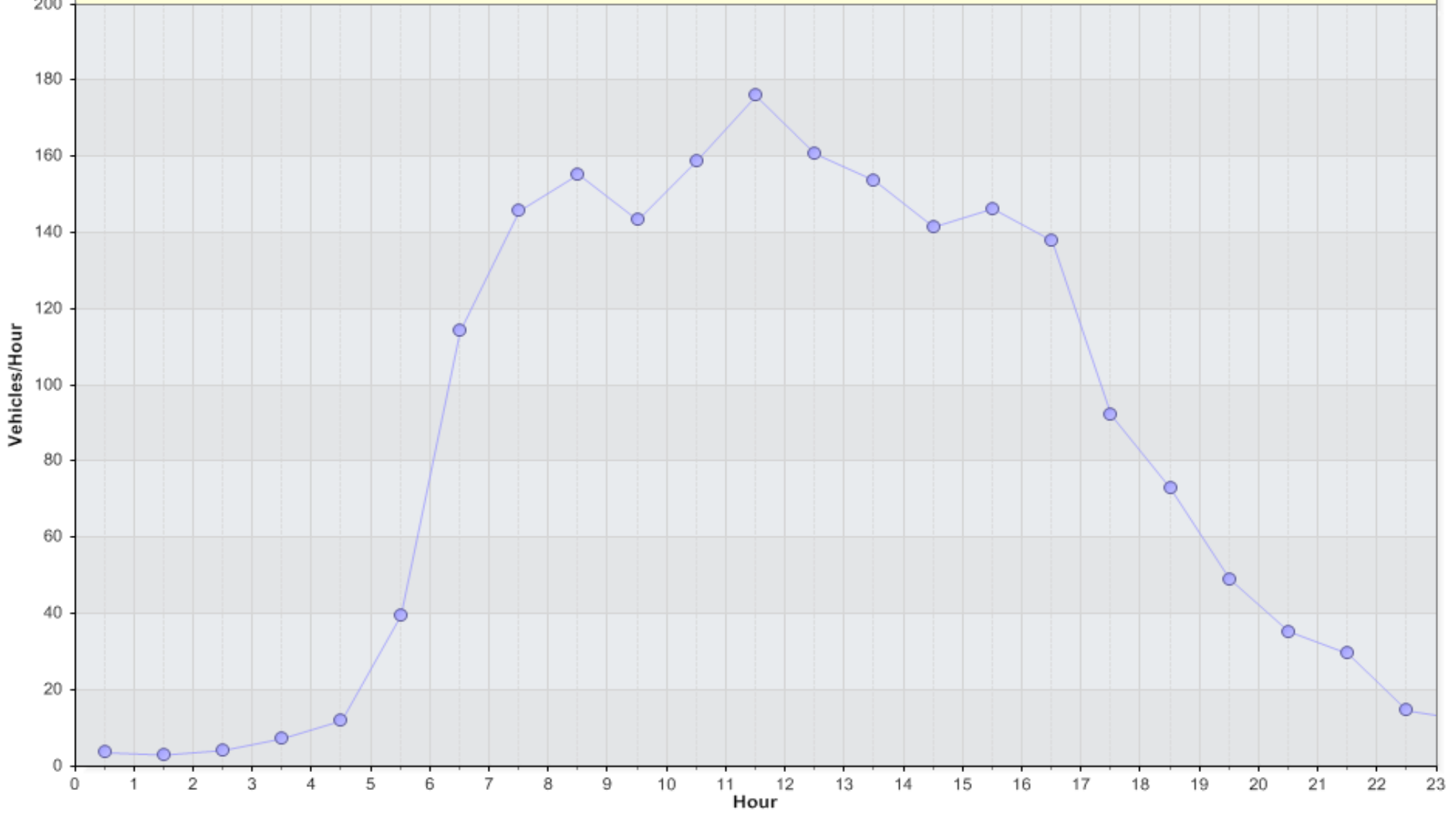
Outbound to Stretham: Average Hourly Volume for Week of 21/12/2020 Average Counts By Hour (21/12/2020) —●— Average Counts By Hour (21/12/2020)
