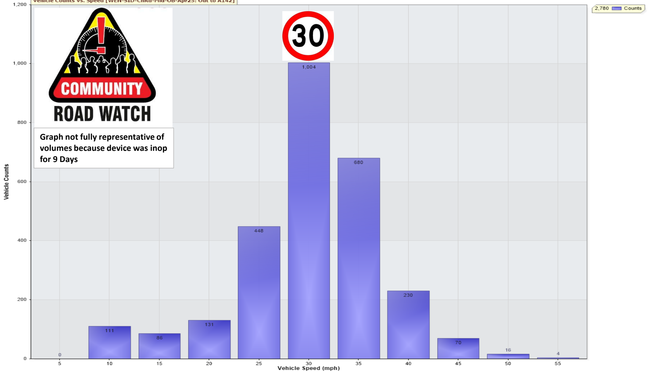
Vehicle Counts Vs. Speed [WEN-SID-ChRd-Mid-OB-Apr25: Out to A142]
