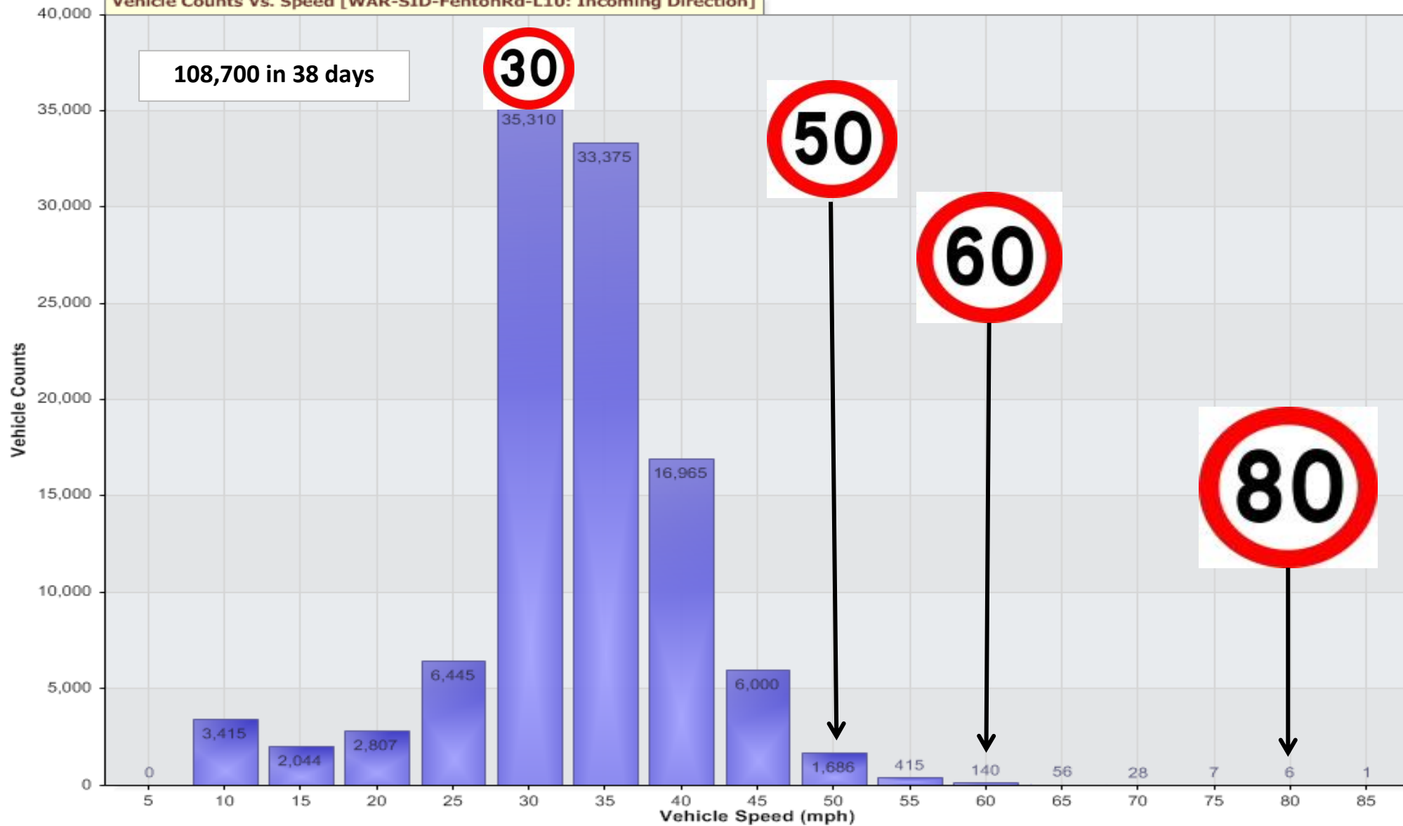
Vehicle Counts Vs. Speed [WAR-SID-FentonRd-L10: Incoming Direction]
