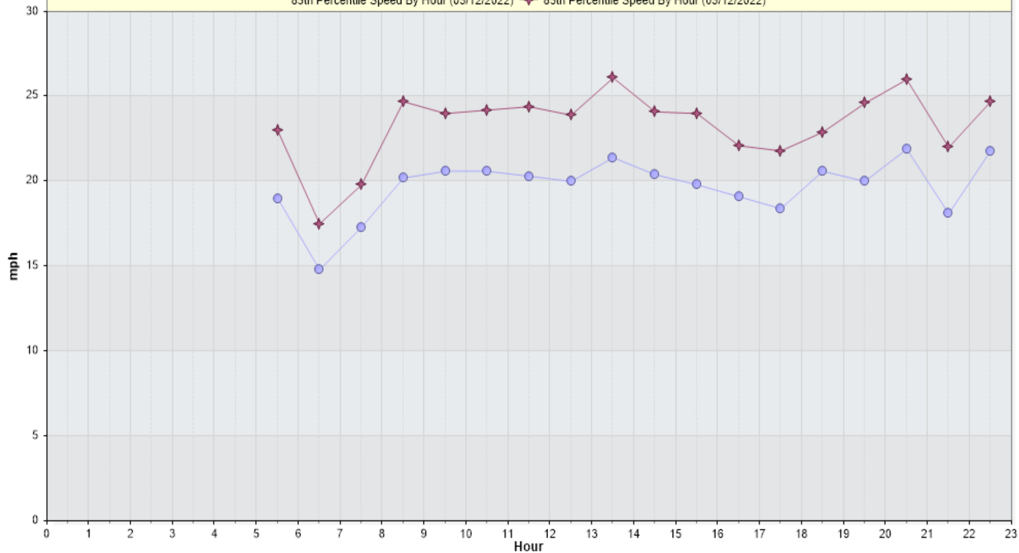
From A1:Average Hourly WEEKDAY Speeds for Week of 05/12/2022 Average Hourly WEEKDAY Speeds By Hour (05/12/2022) — Average Hourly WEEKDAY Speeds By Hour (05/12/2022) 85th Percentile Speed By Hour (05/12/2022) — 85th Percentile Speed By Hour (05/12/2022)
