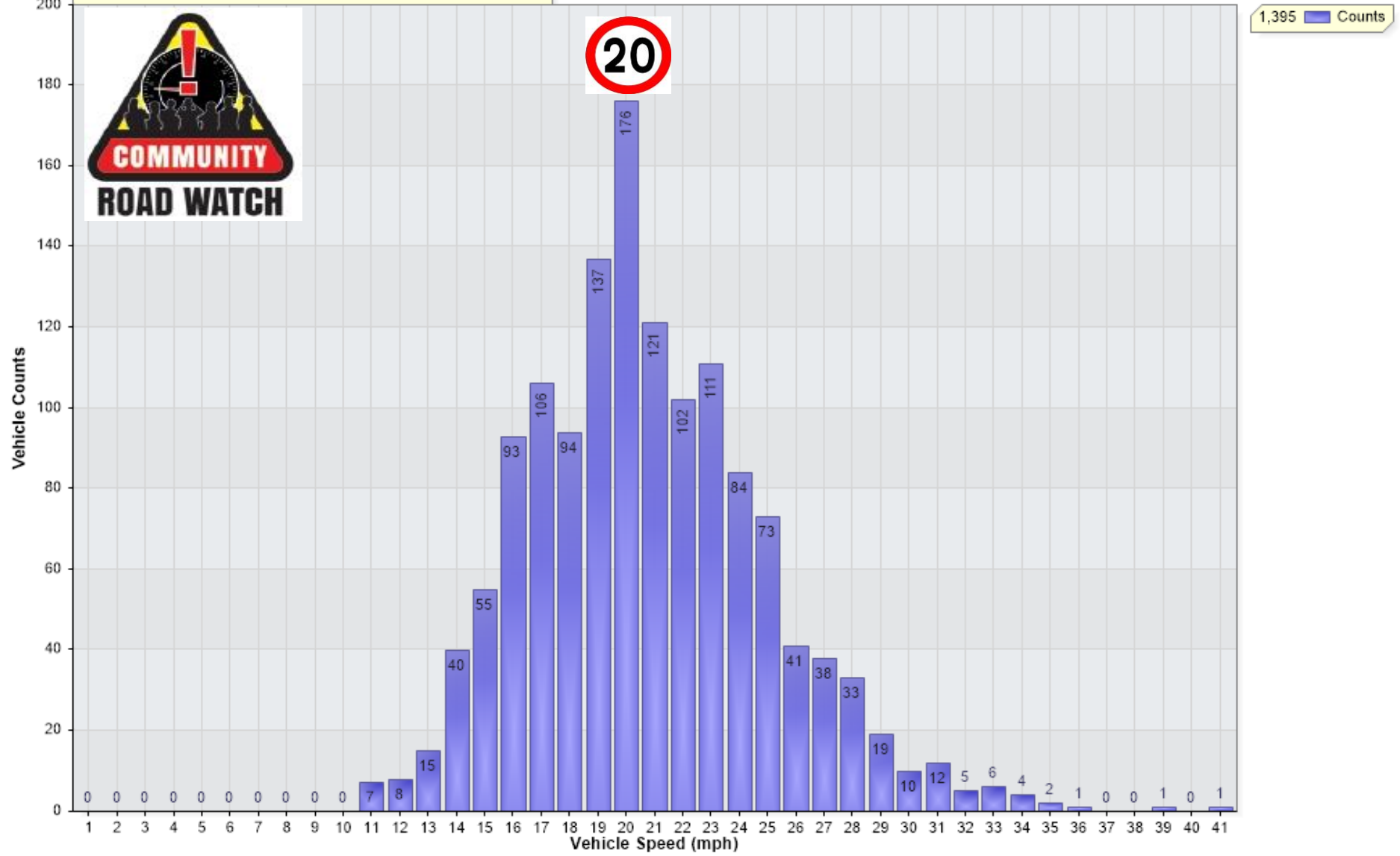
Vehicle Counts Vs. Speed [Log-UPT-MainRd-Dec22: From A1]
