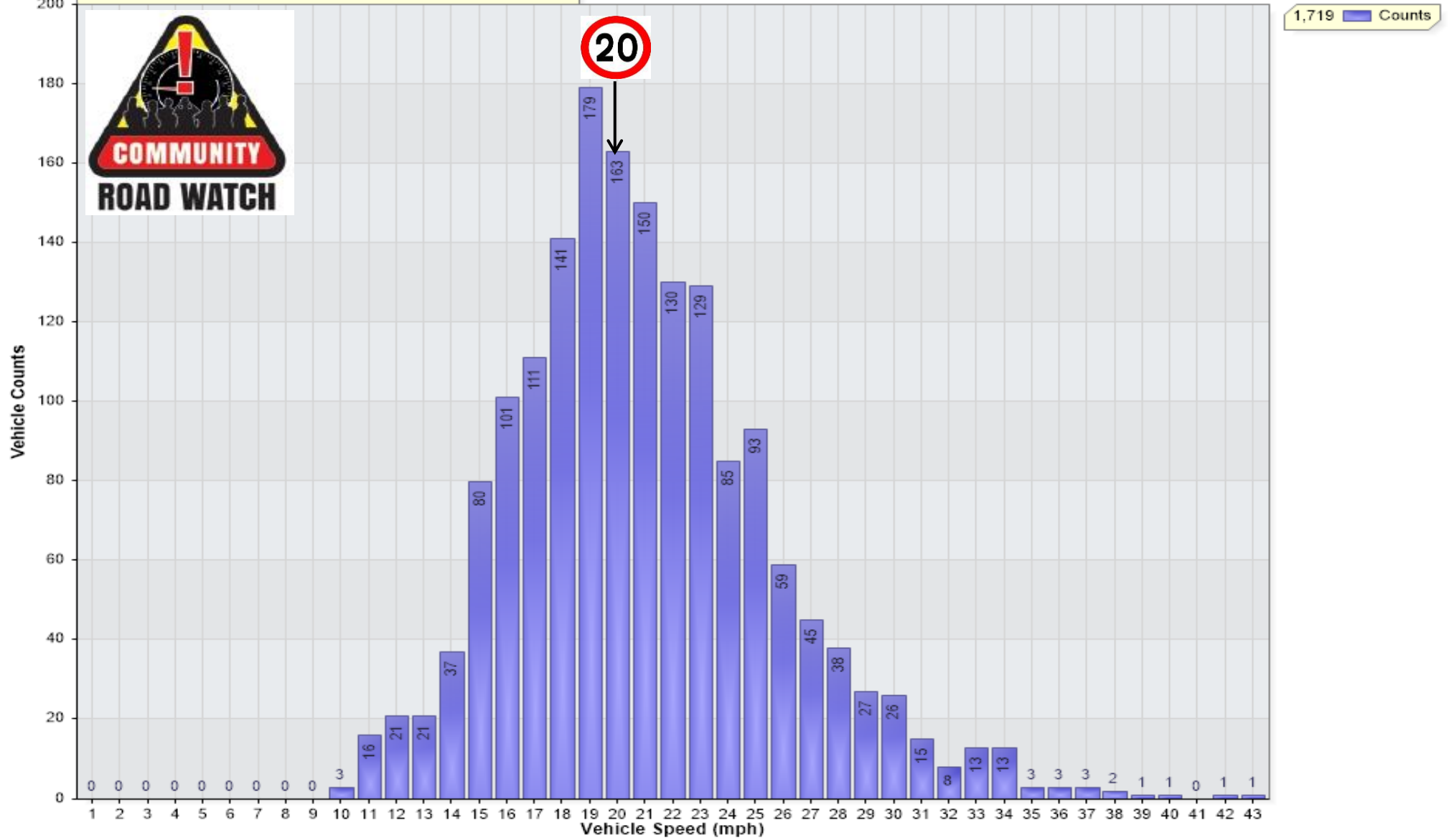
Vehicle Counts Vs. Speed [Log-UPT-MainRd-Dec22: To A1]
