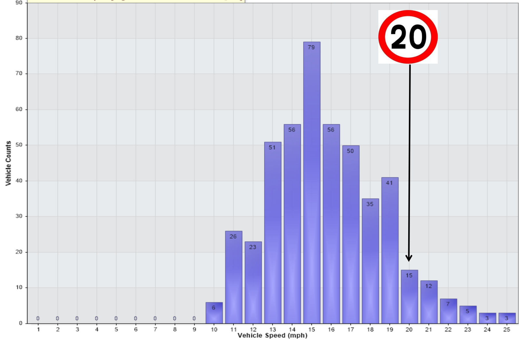
Vehicle Counts Vs. Speed [LogUPT-GrnLnAtVH-Dec22: Down @ VH]
