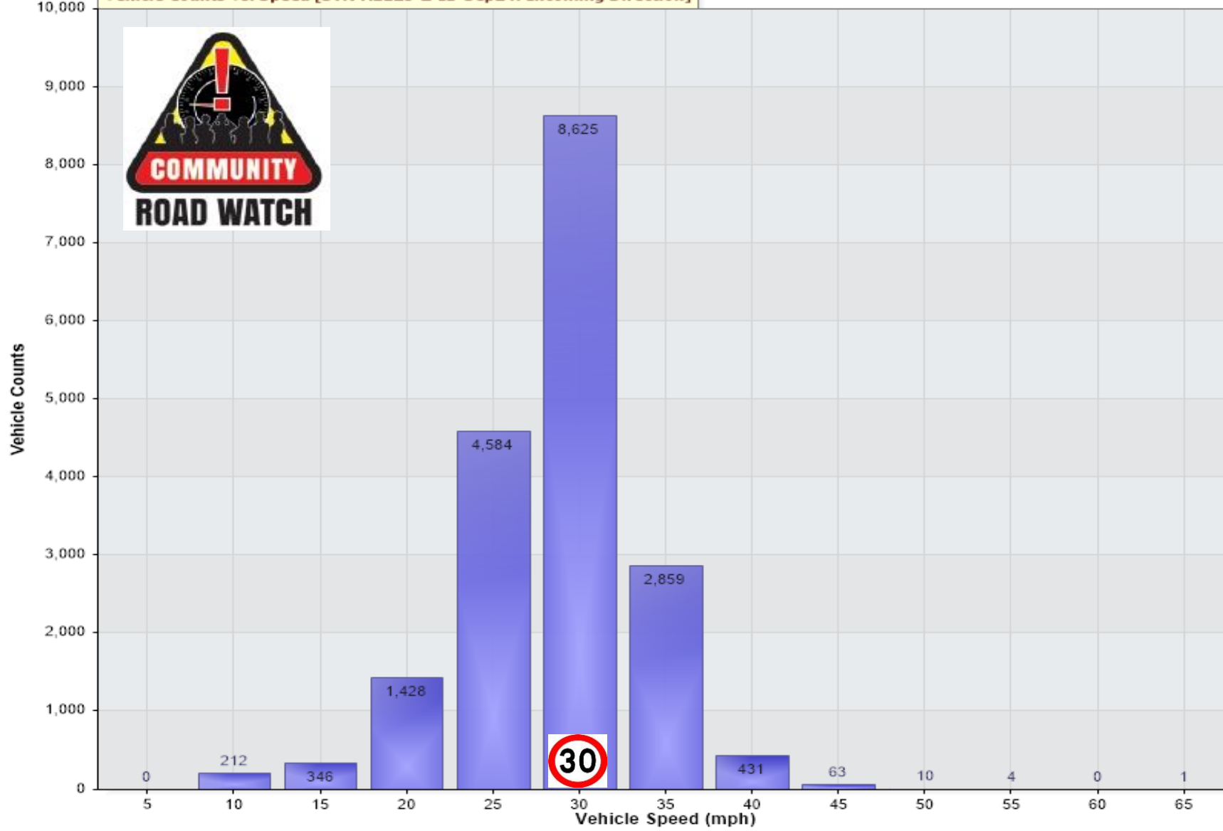
Vehicle Counts Vs. Speed [STR-A1123-Z-IB-Sep24: Incoming Direction]
