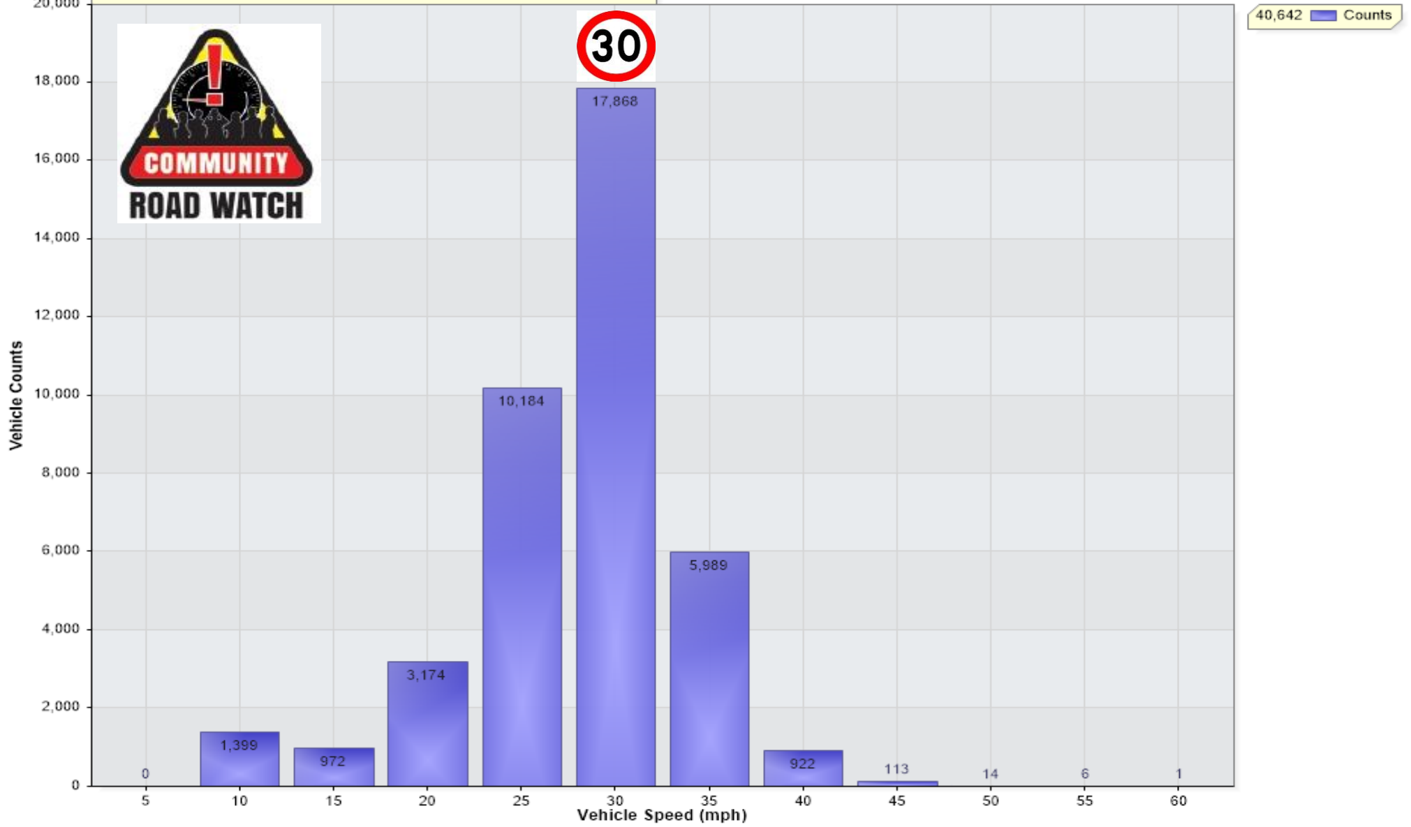
Vehicle Counts Vs. Speed [STR-A1123-Z-IB-Sep24: Incoming Direction]
