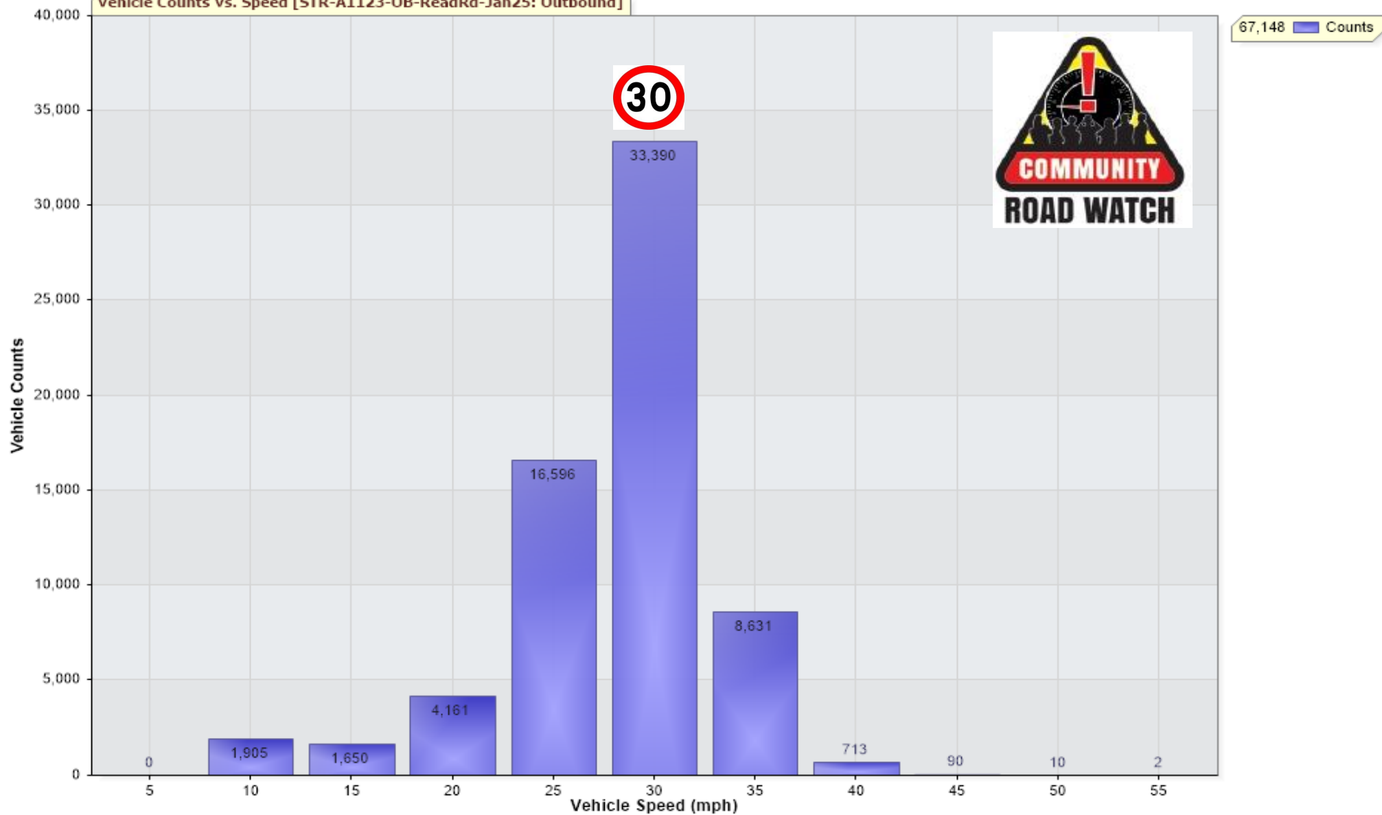
Vehicle Counts Vs. Speed [STR-A1123-OB-ReadRd-Jan25: Outbound]
