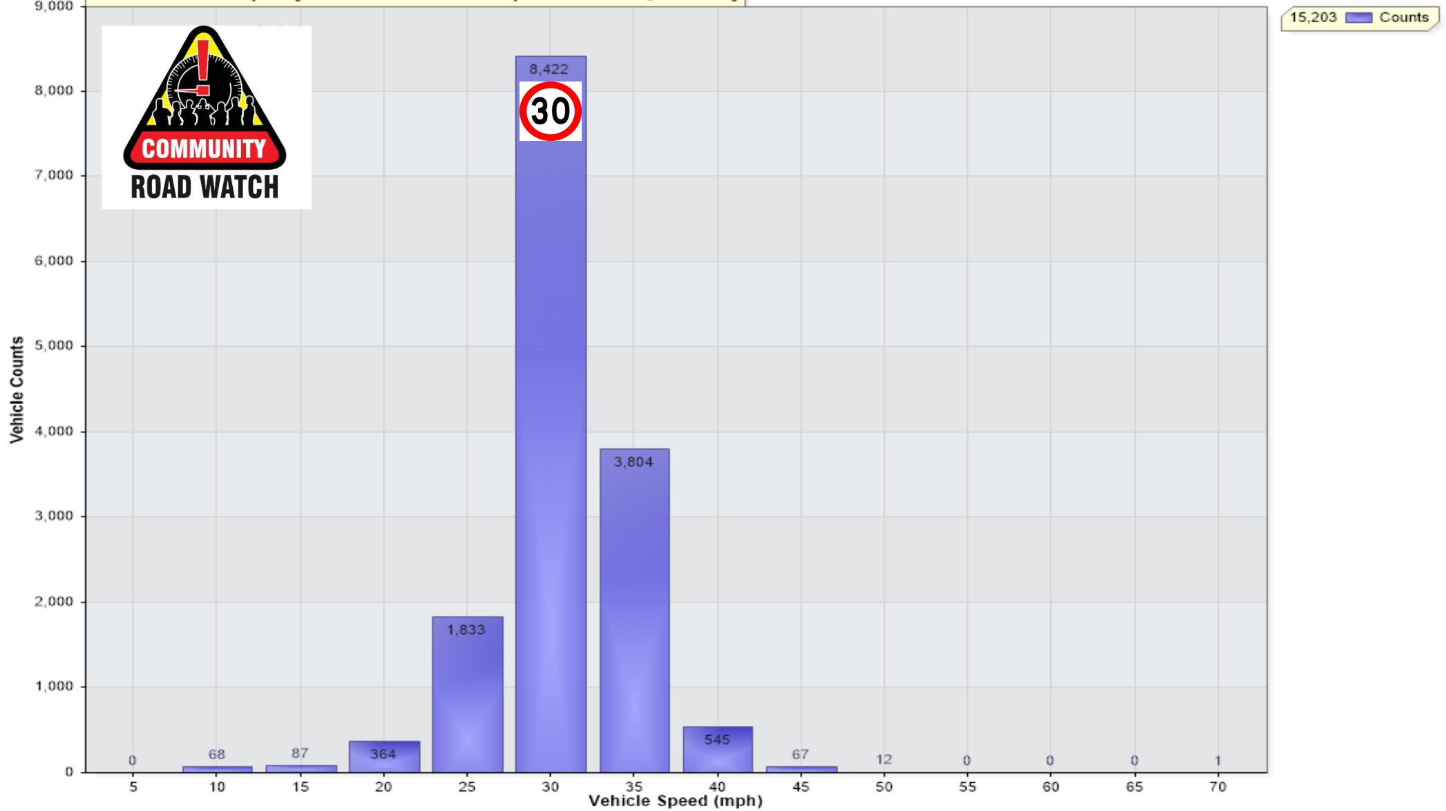
Vehicle Counts Vs. Speed [STR-A1123-Stennett-OB-Apr25: Outbound @ Stennett]
