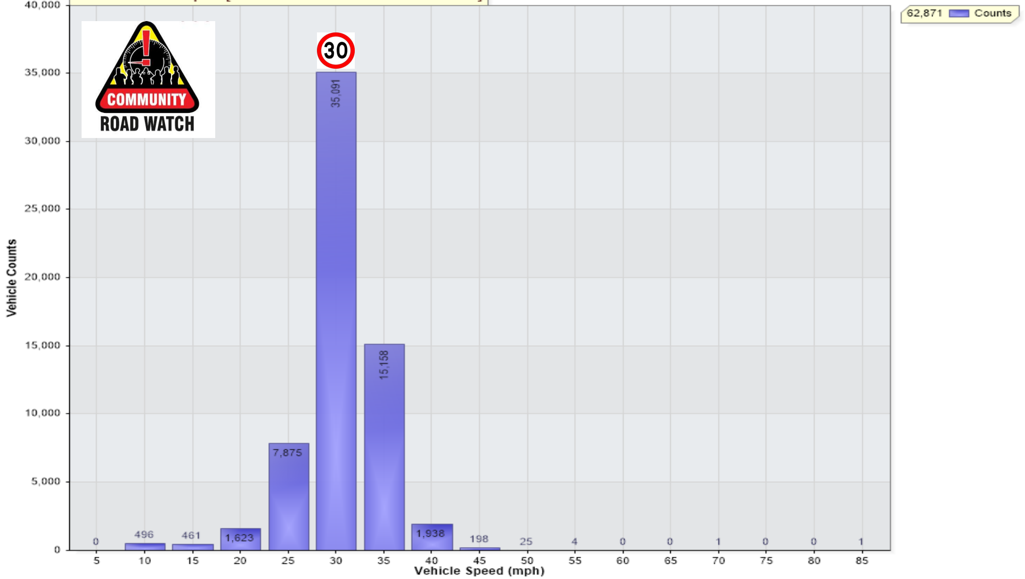
Vehicle Counts Vs. Speed [STR-A1123-OB-Sennitt-Mar25: Outbound]
