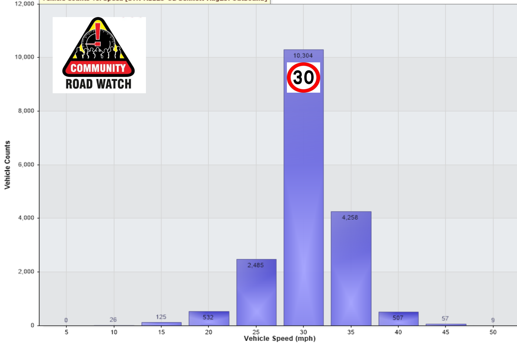
Vehicle Counts Vs. Speed [STR-A1123-OB Sennett-Aug25: Outbound]
