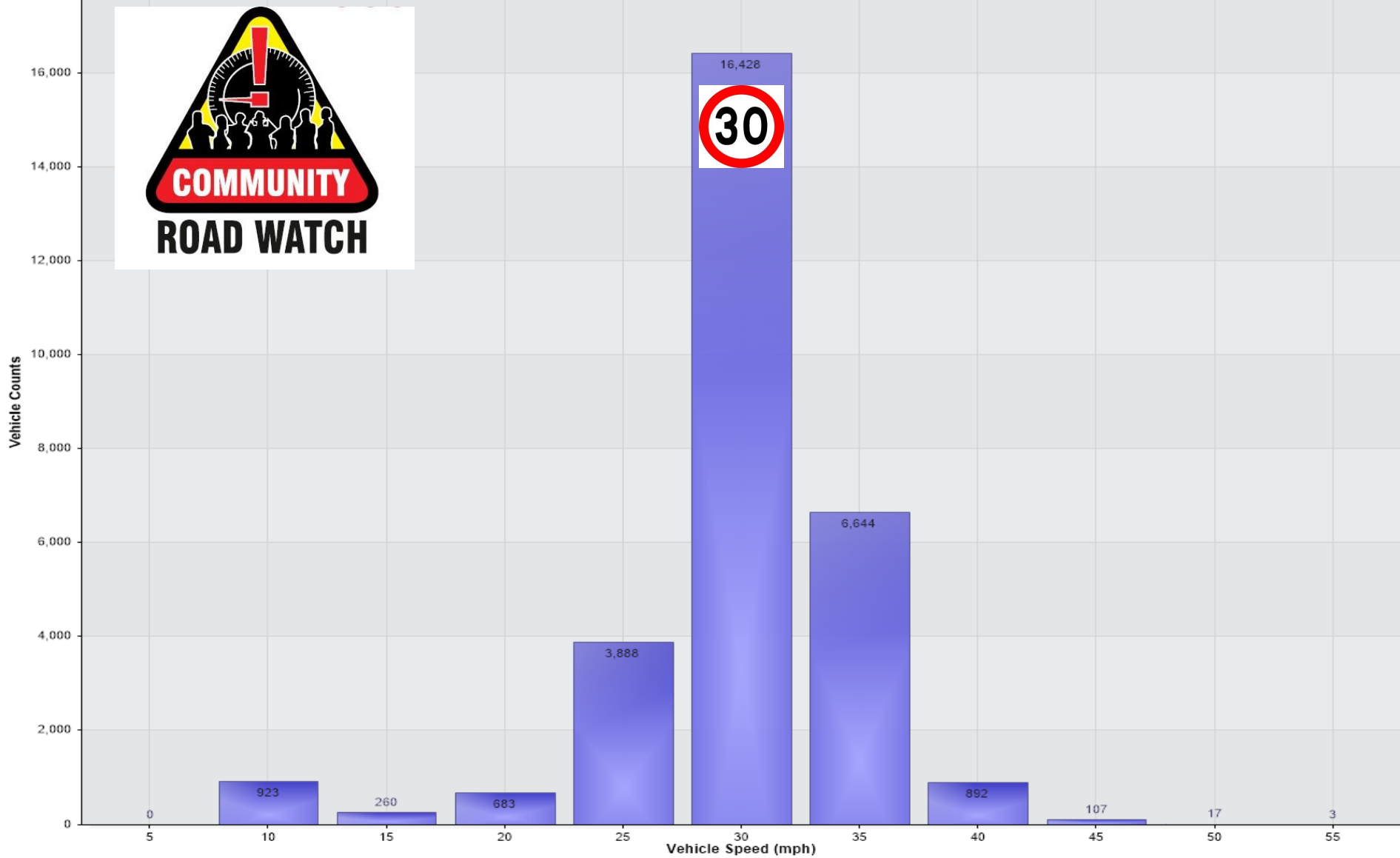
Vehicle Counts Vs. Speed [STR-A1123-OB Sennett-Jul25: Outbound]
