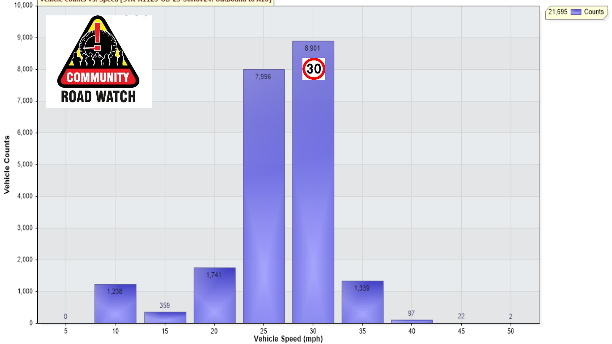
Vehicle Counts Vs. Speed [STR-A1123-OB-25-30Nov24: Outbound to A10]
