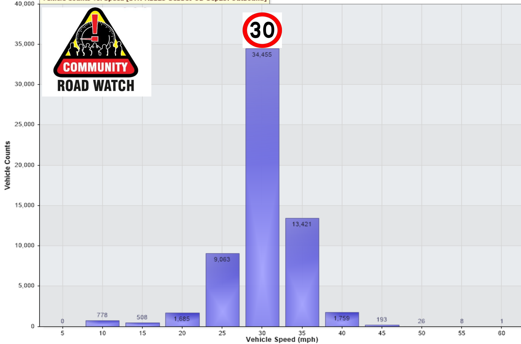
Vehicle Counts Vs. Speed [STR-A1123-Sebbet-OB-Sep25: Outbound]
