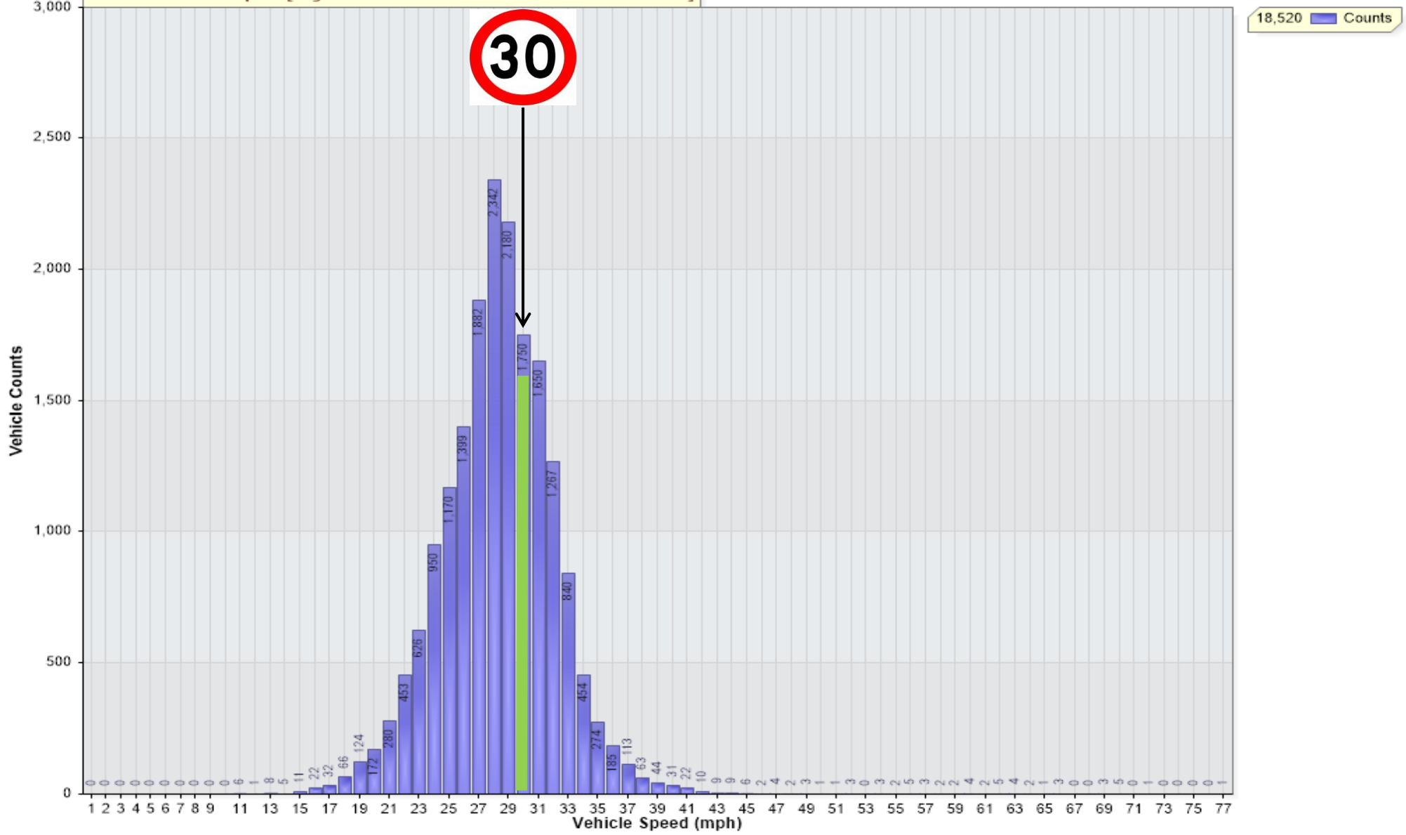
Vehicle Counts Vs. Speed [LogSTR-A1123-AtGarden: A1123 Inbound On Bend]
