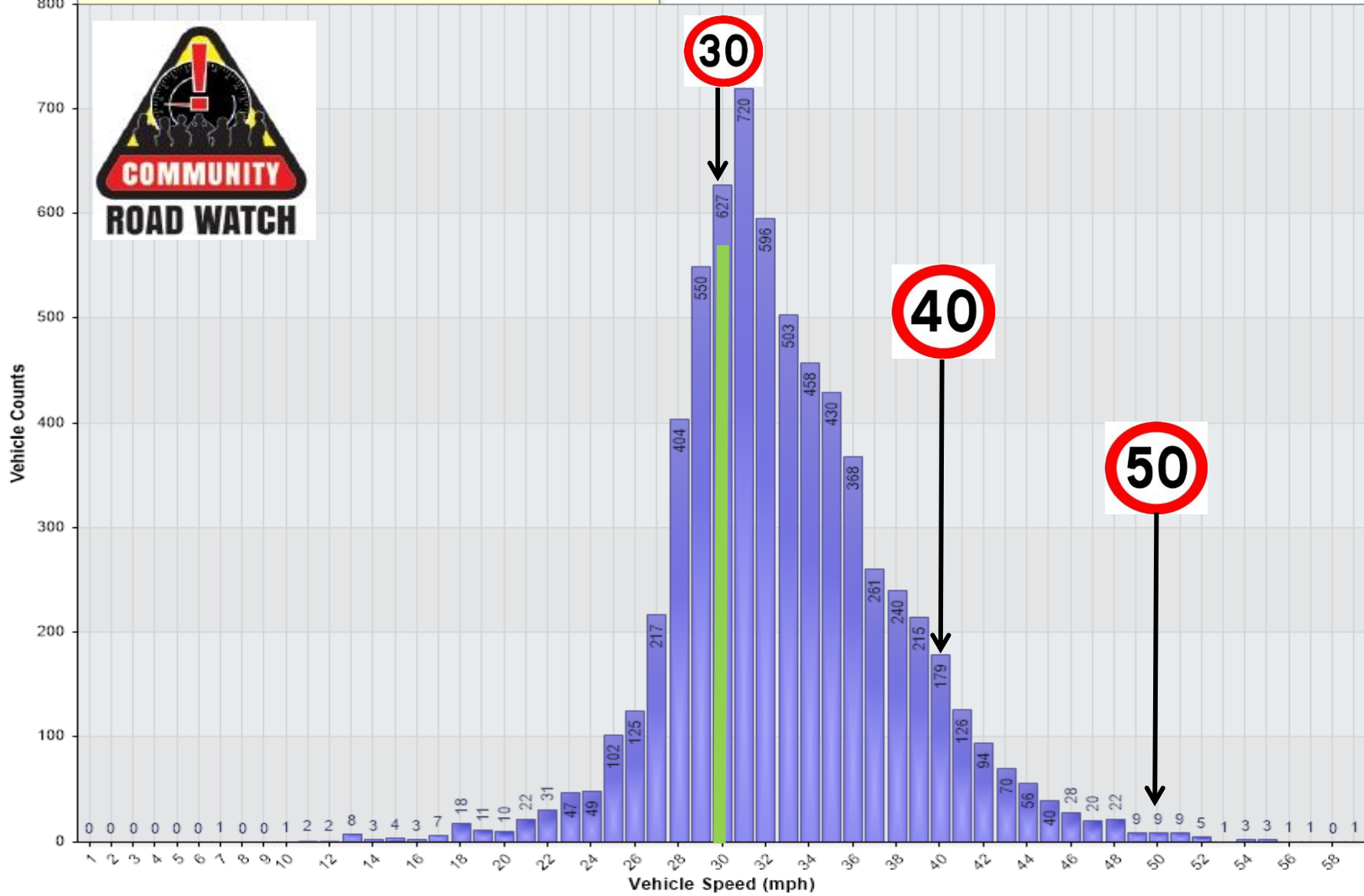
Vehicle Counts Vs. Speed [LogSTO-FIB-Sep24: Incoming Direction]
