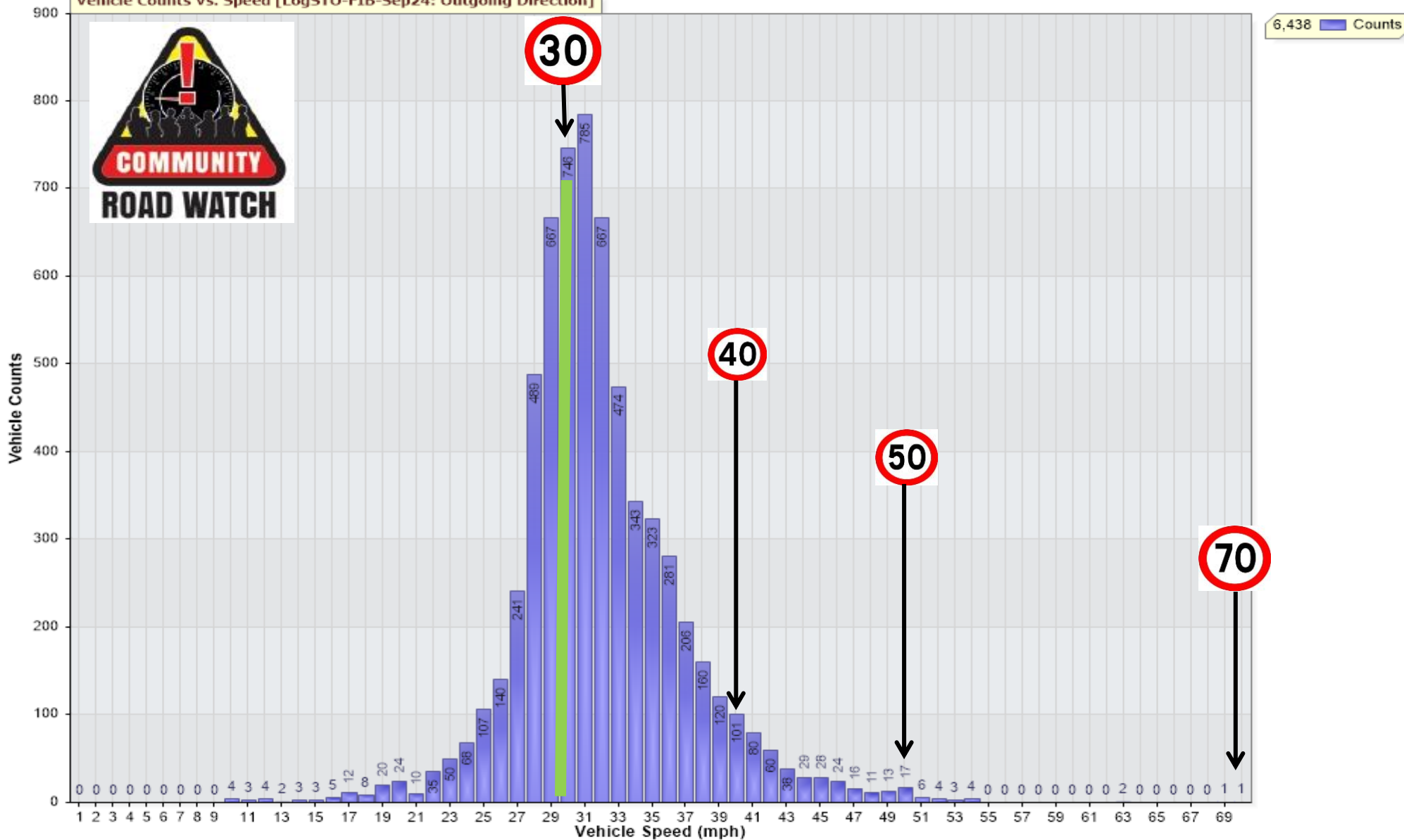
Vehicle Counts Vs. Speed [LogSTO-FIB-Sep24: Outgoing Direction]
