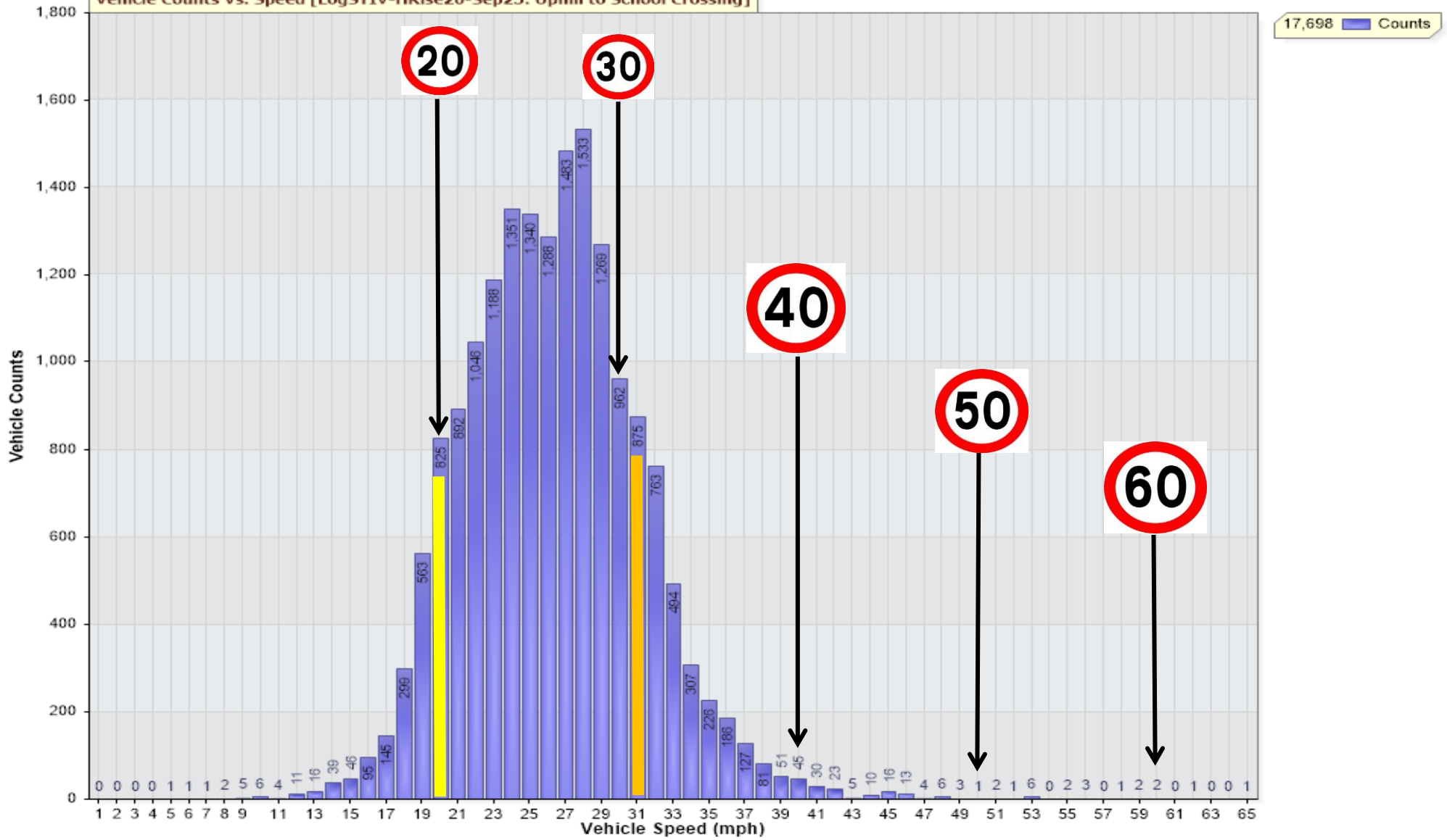
Vehicle Counts Vs. Speed [LogSTIV-HRise20-Sep23: Uphill to School Crossing]
