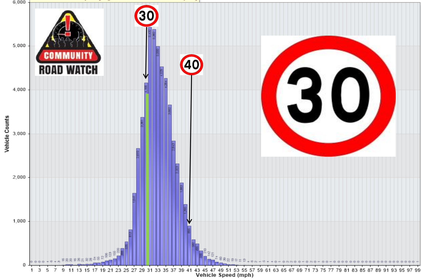
Vehicle Counts Vs. Speed [LogSIV-A1123-How30-Jul24: Uphill]
