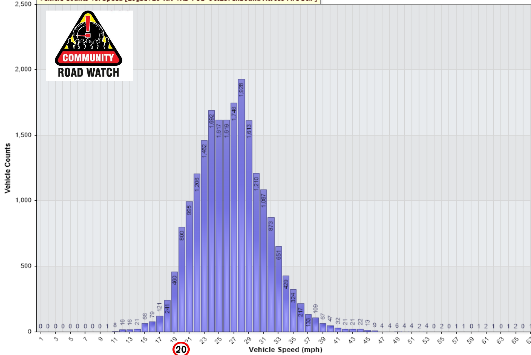
Vehicle Counts Vs. Speed [LogSIV20-RR-VAS-FOB-Oct25: Inbound Across Fire Stn ]
