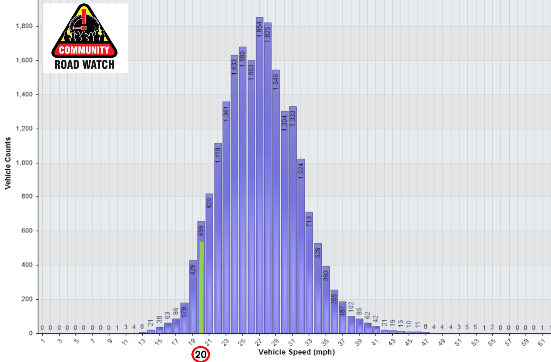
Vehicle Counts Vs. Speed [LogSIV20-RR-VAS-FOB-Oct25: OutBound at Slepe Hall]
