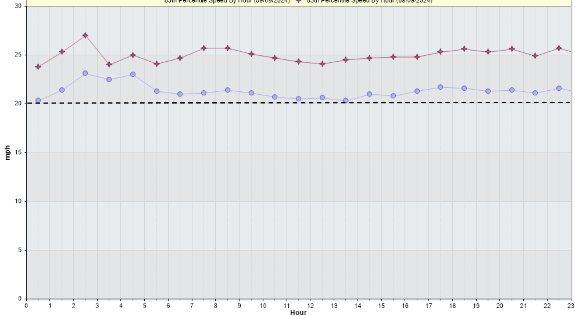
Merged:Average Hourly WEEKDAY Speeds for Week of 09/09/2024 Average Hourly WEEKDAY Speeds By Hour (09/09/2024) —●— Average Hourly WEEKDAY Speeds By Hour (09/09/2024) 85th Percentile Speed By Hour (09/09/2024) —◆— 85th Percentile Speed By Hour (09/09/2024)
