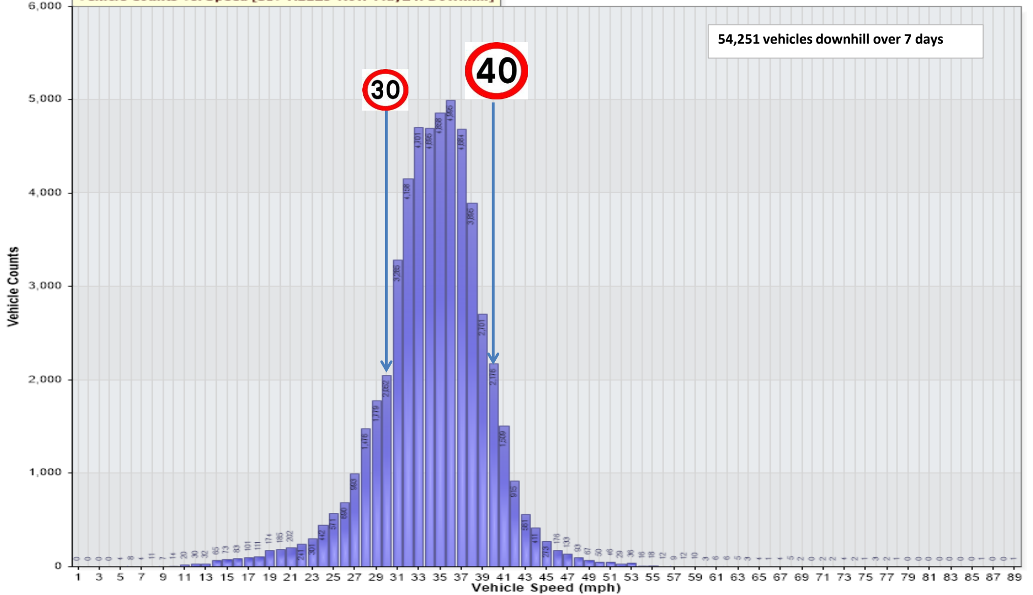
Vehicle Counts Vs. Speed [SIV-A1123-How-May24: Downhill]
