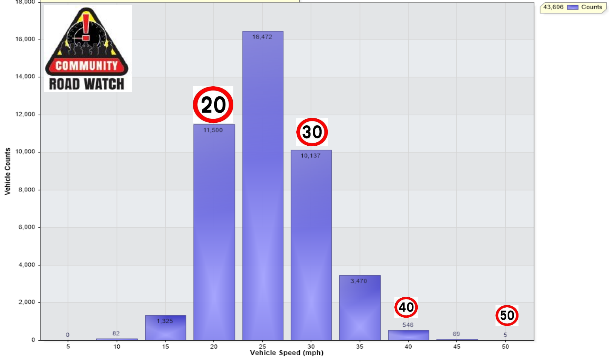
Vehicle Counts Vs. Speed [SOM-SWO-HiStIB-SepOct23: Incoming Direction]
