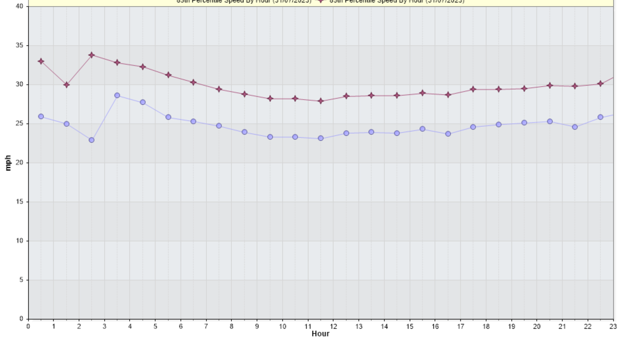
Outbound: Average Hourly WEEKDAY Speeds for Week of 31/07/2023 Average Hourly WEEKDAY Speeds By Hour (31/07/2023) — Average Hourly WEEKDAY Speeds By Hour (31/07/2023) 85th Percentile Speed By Hour (31/07/2023) — 85th Percentile Speed By Hour (31/07/2023)
