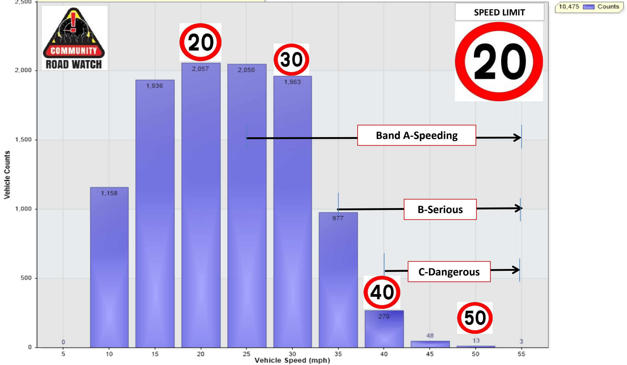
Vehicle Counts Vs. Speed [SOM20-ChRd-OB-Jan24: To Chatteris]
