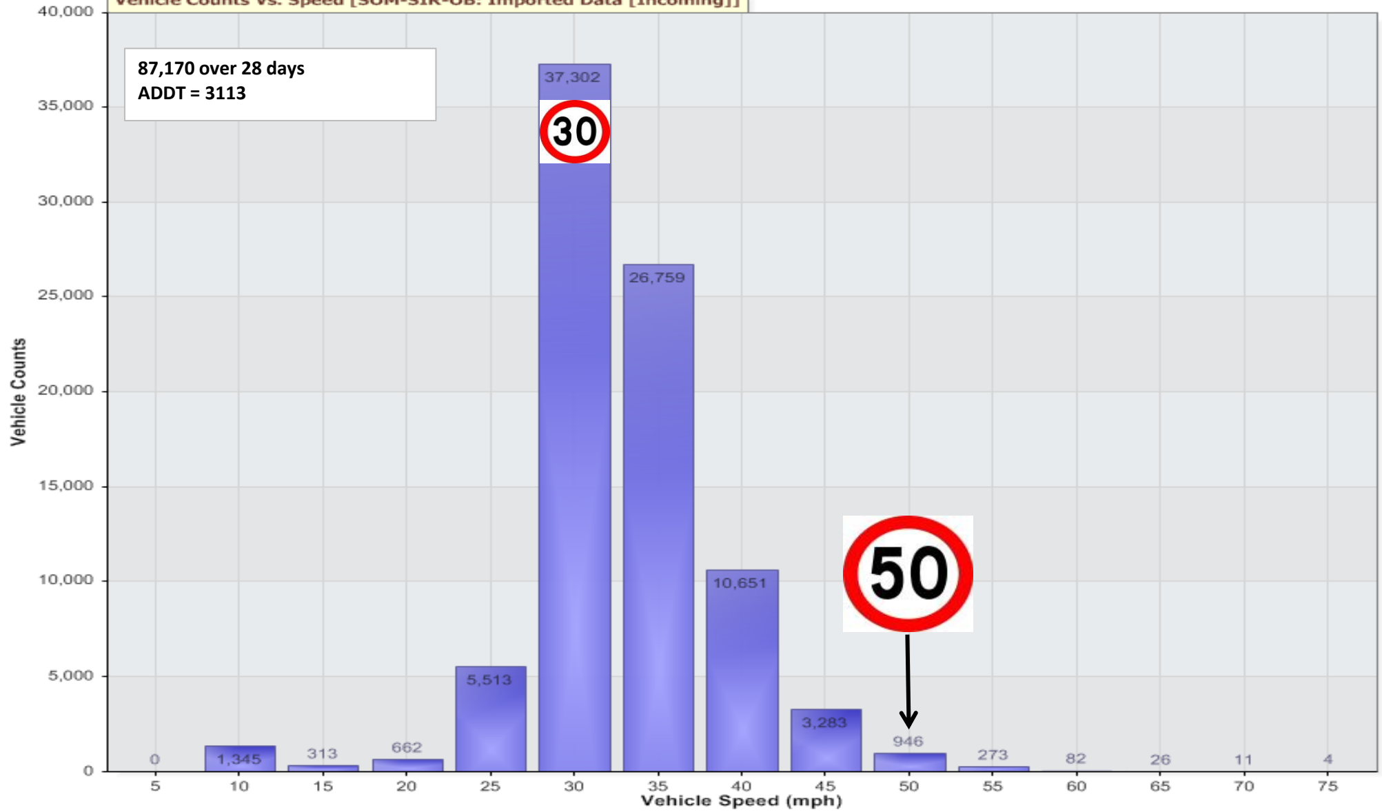
Vehicle Counts Vs. Speed [SOM-SIR-OB: Imported Data [Incoming]]
