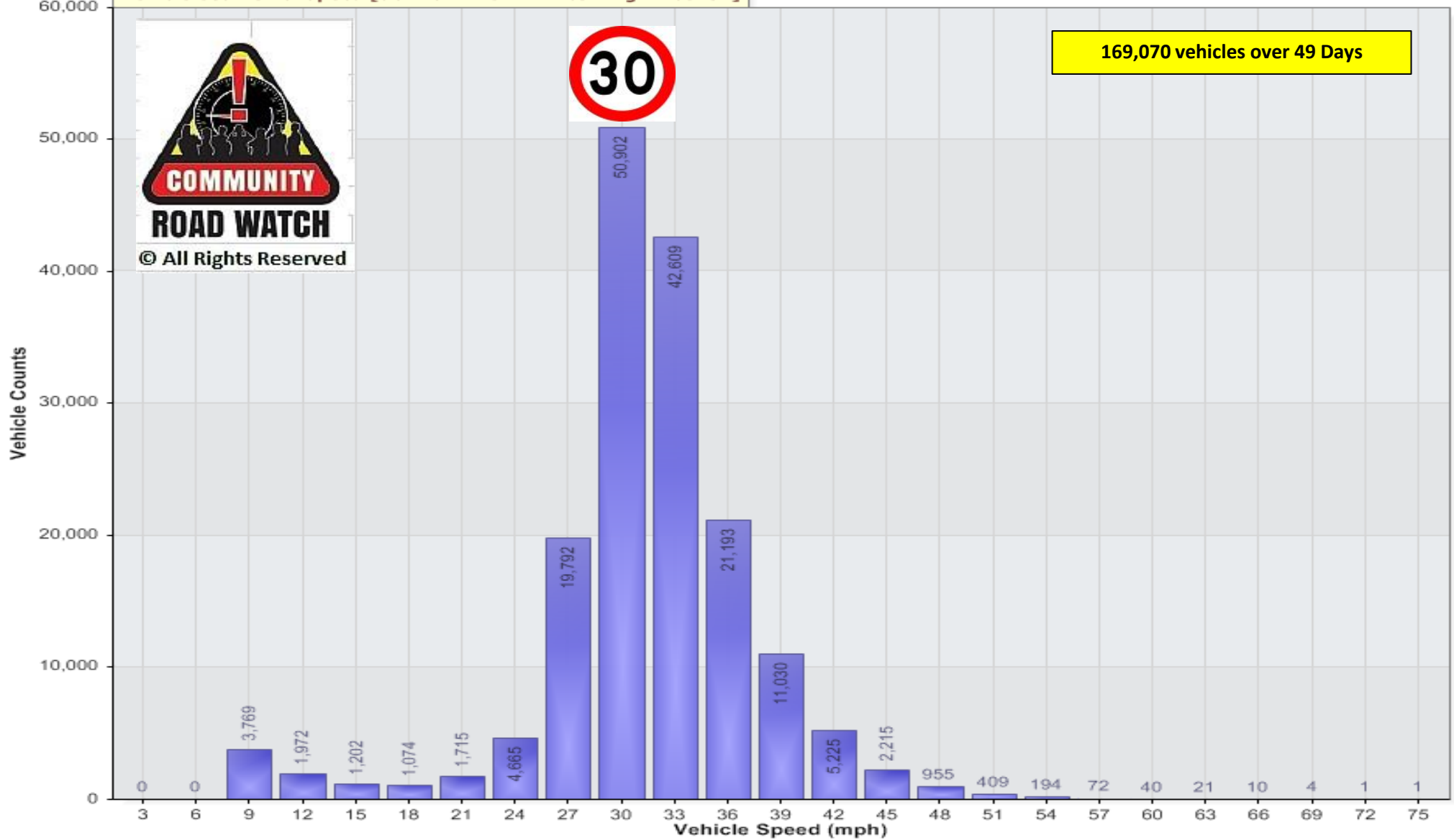
Vehicle Counts Vs. Speed [SOM-SIRAt6-IB: Incoming Direction]
