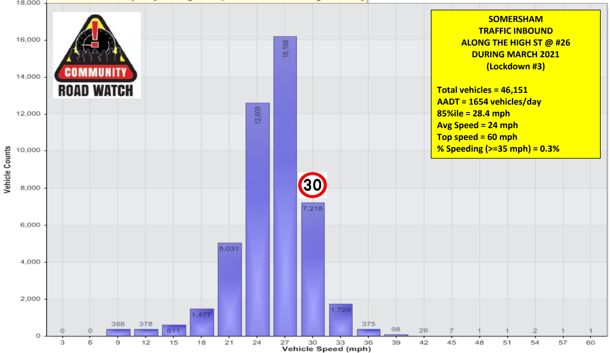
Vehicle Counts Vs. Speed [SOM-HighSt-IB@No26-Mar21: Incoming Direction]
