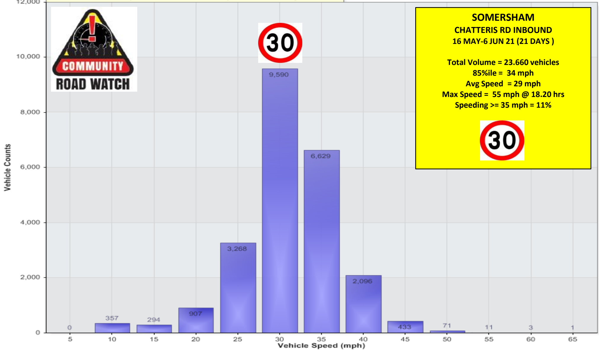
Vehicle Counts Vs. Speed [SOM-CHRD-IB-MayJun21: Incoming Direction]
