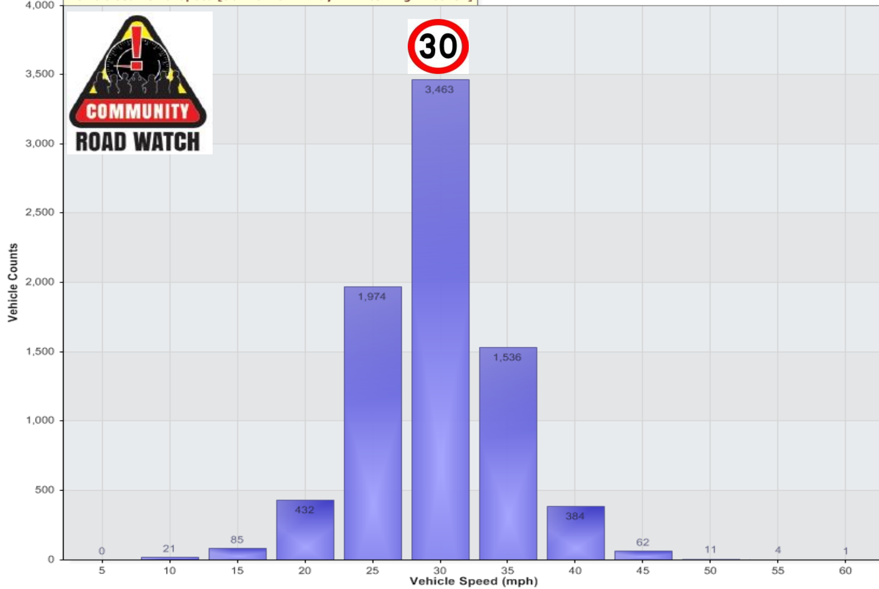
Vehicle Counts Vs. Speed [SOM-ChRd-IB-May22: Incoming Direction]
