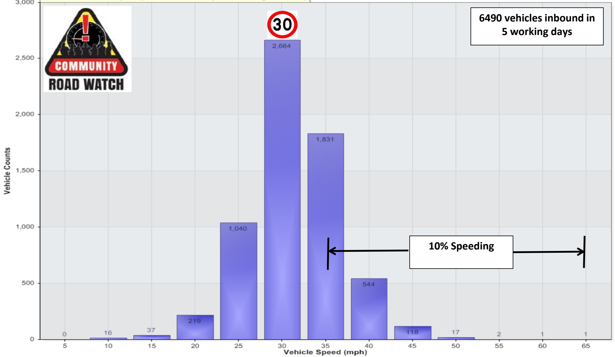
Vehicle Counts Vs. Speed [SOM-ChRd-IB-May22: Incoming Direction]
