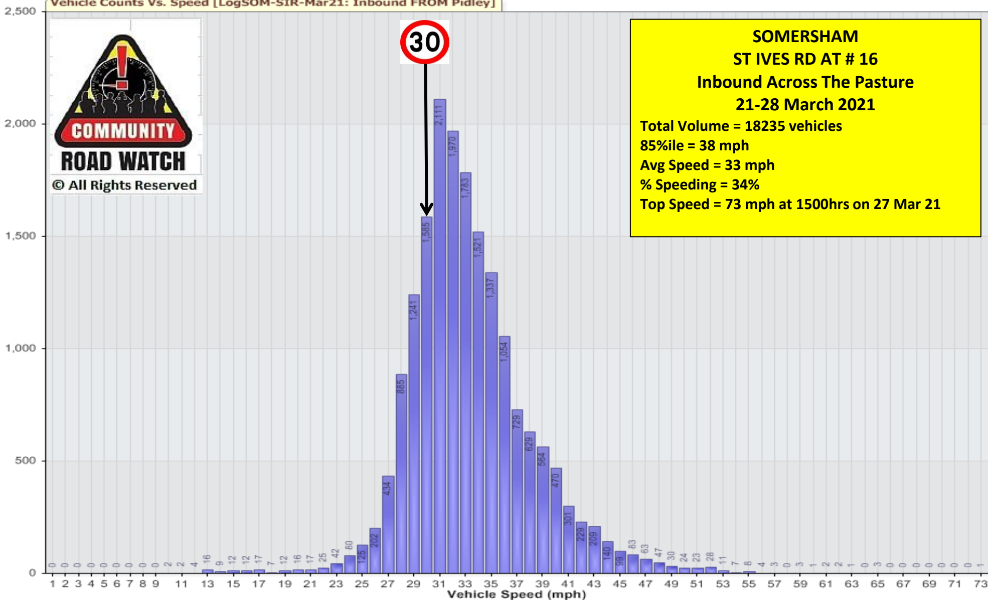
Vehicle Counts Vs. Speed [LogSOM-SIR-Mar21: Inbound FROM Pidley]
