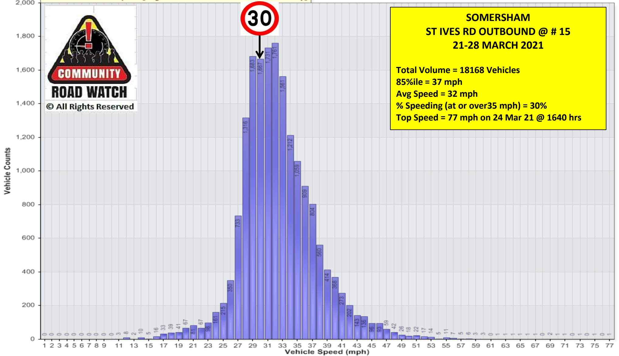
Vehicle Counts Vs. Speed [LogSOM-SIR-Mar21: Outbound TO Pidley]
