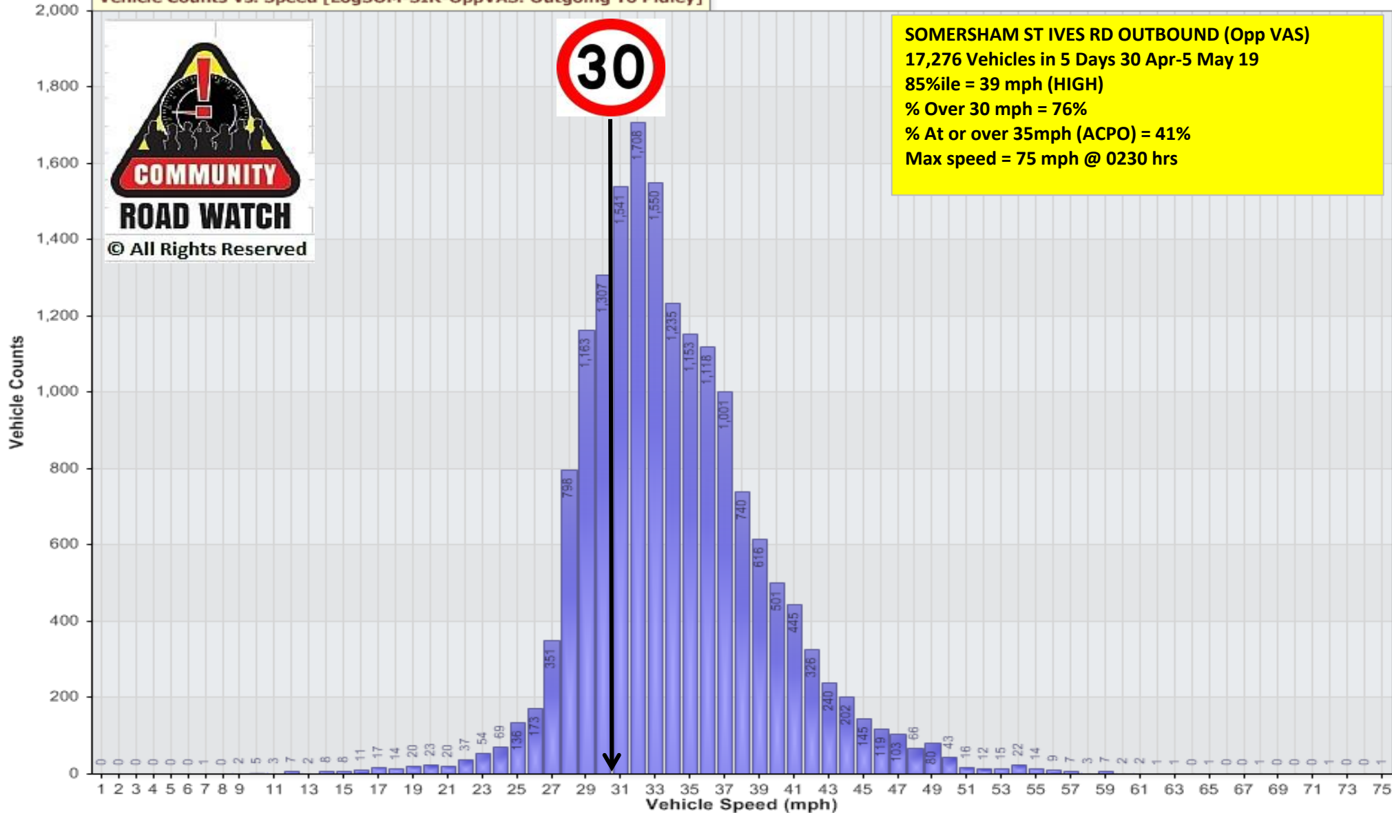
Vehicle Counts Vs. Speed [LogSOM-SIR-OppVAS: Outgoing To Pidley]
