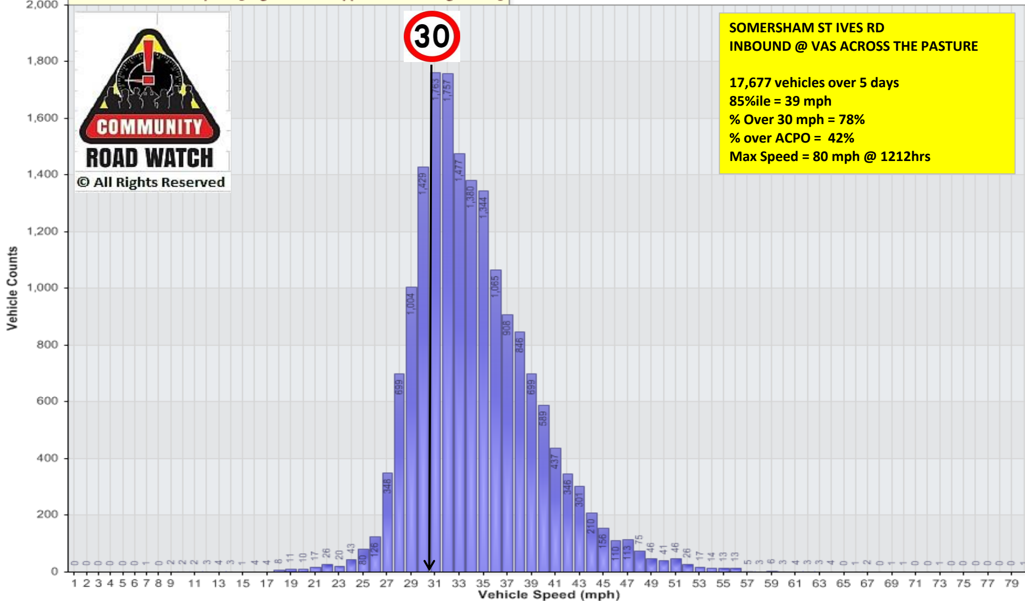
Vehicle Counts Vs. Speed [LogSOM-SIR-OppVAS: Incoming + VAS]
