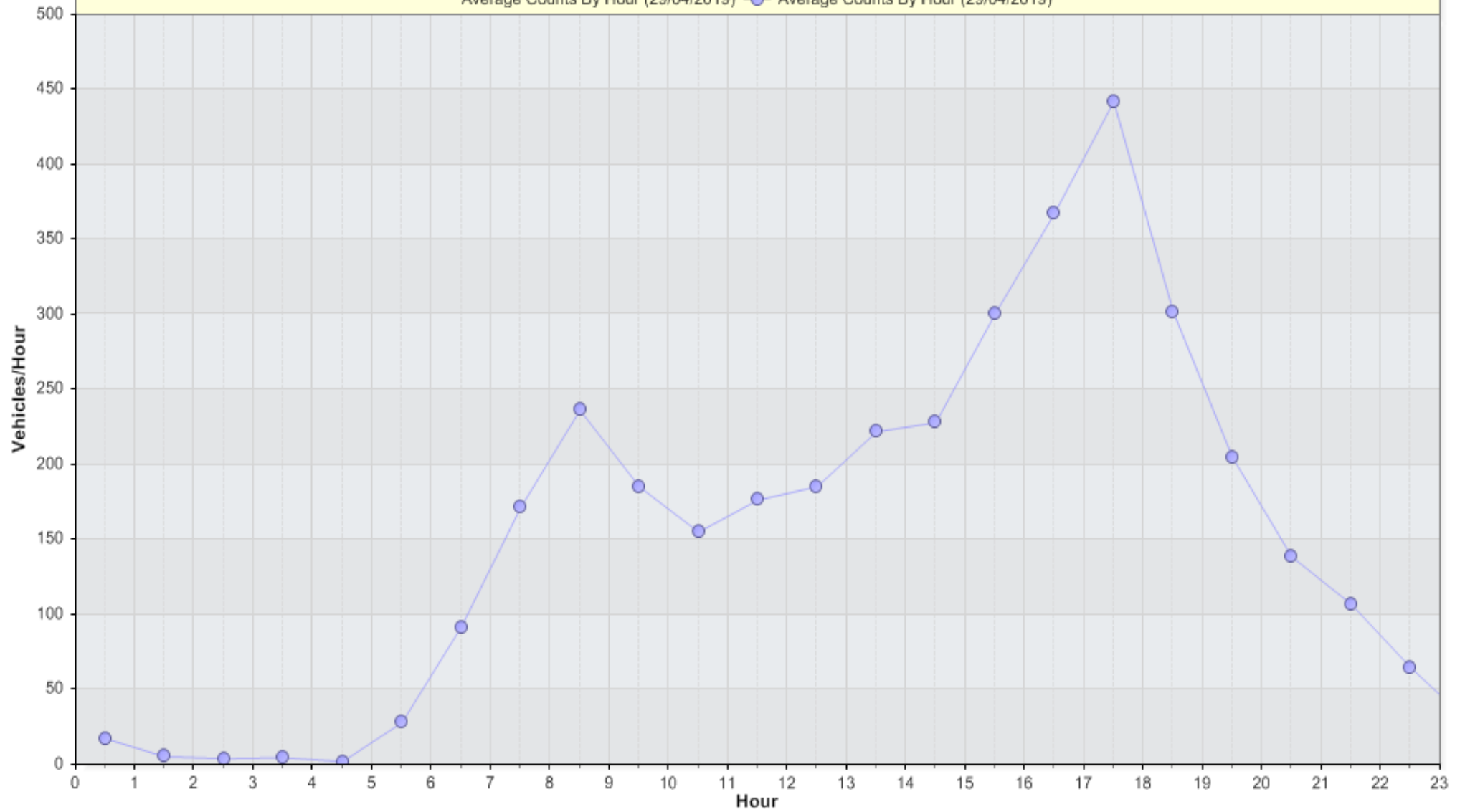
Incoming + VAS:Average Hourly Volume for Week of 29/04/2019 Average Counts By Hour (29/04/2019) —●— Average Counts By Hour (29/04/2019)
