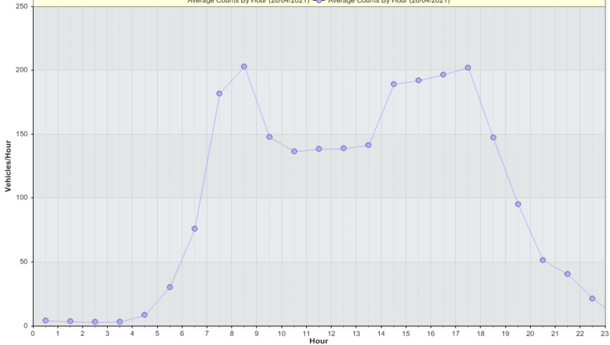
Inbound from Colne: Average Hourly Volume for Week of 26/04/2021 Average Counts By Hour (26/04/2021) —●— Average Counts By Hour (26/04/2021)
