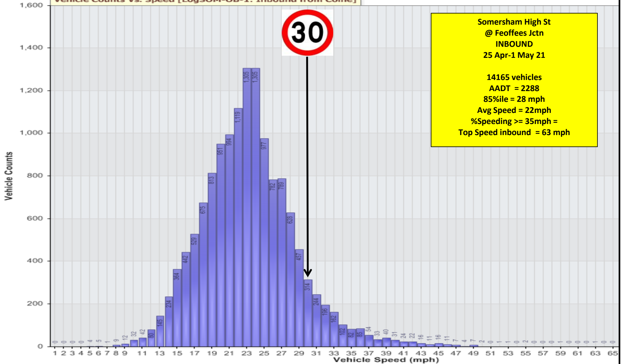
Vehicle Counts Vs. Speed [LogSOM-OB-1: Inbound from Colne]
