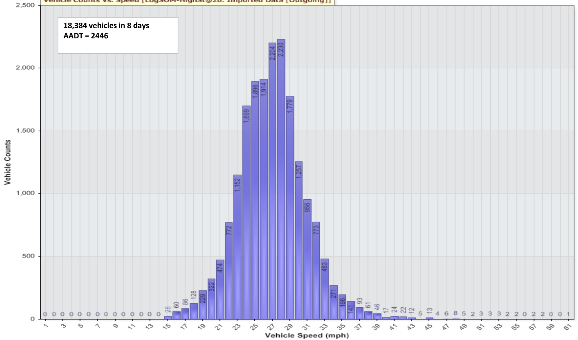
Vehicle Counts Vs. Speed [LogSOM-HighSt@26: Imported Data [Outgoing]]
