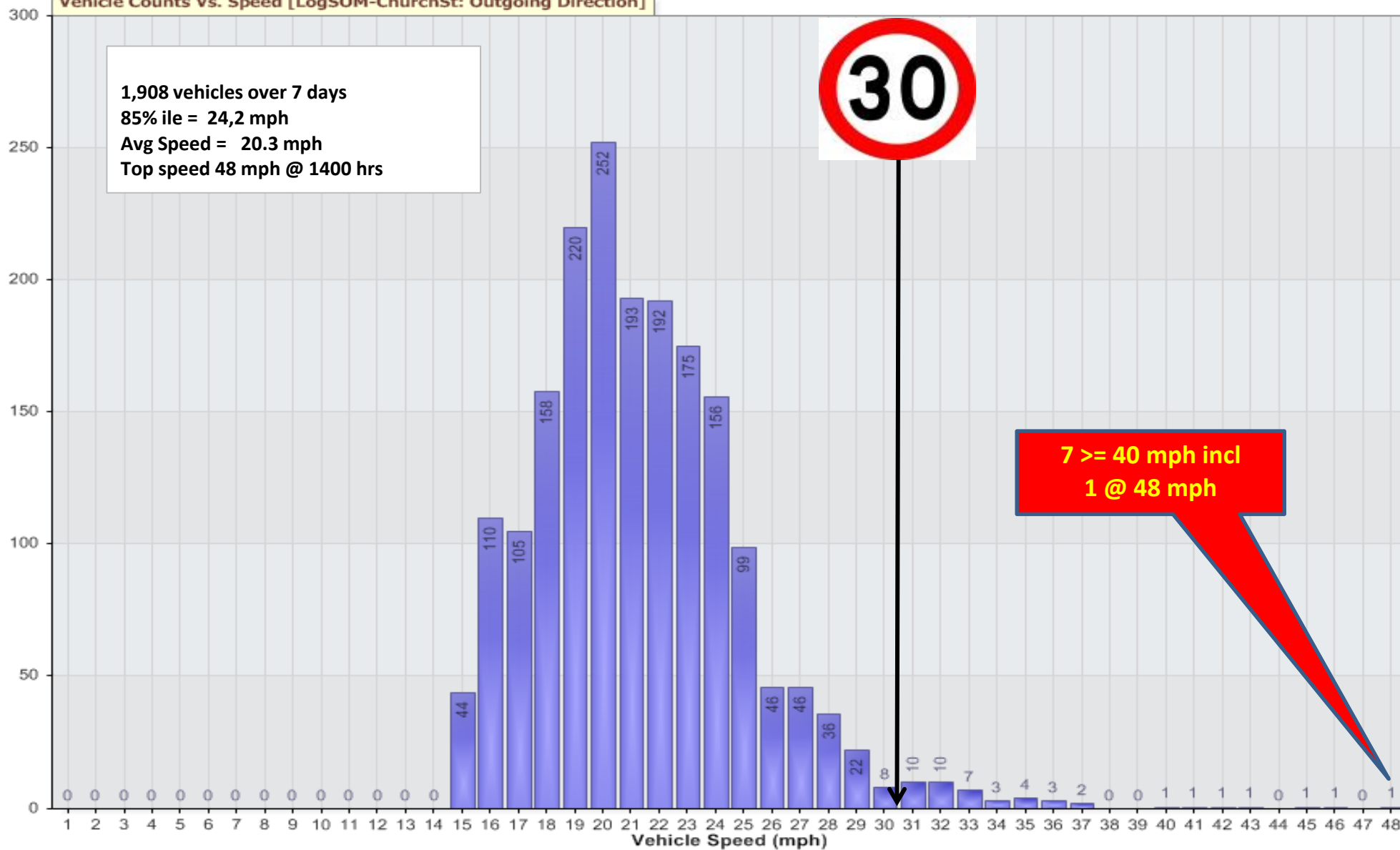
Vehicle Counts Vs. Speed [LogSOM-ChurchSt: Outgoing Direction]
