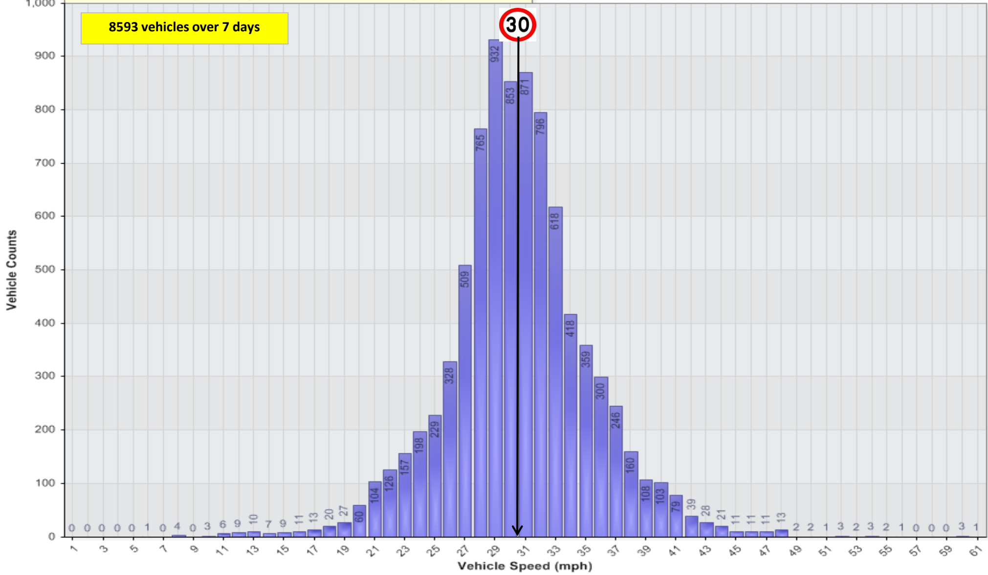
Vehicle Counts Vs. Speed [LogSOM-ChatterisRd-29: Outgoing to Chatteris]
