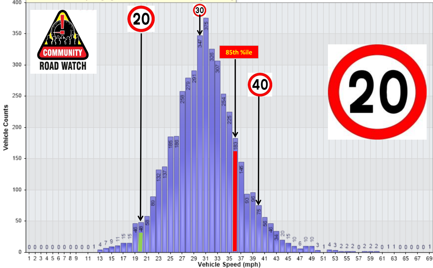
Vehicle Counts Vs. Speed [LogSOM-ChRd20-Dec24: Incoming Direction]
