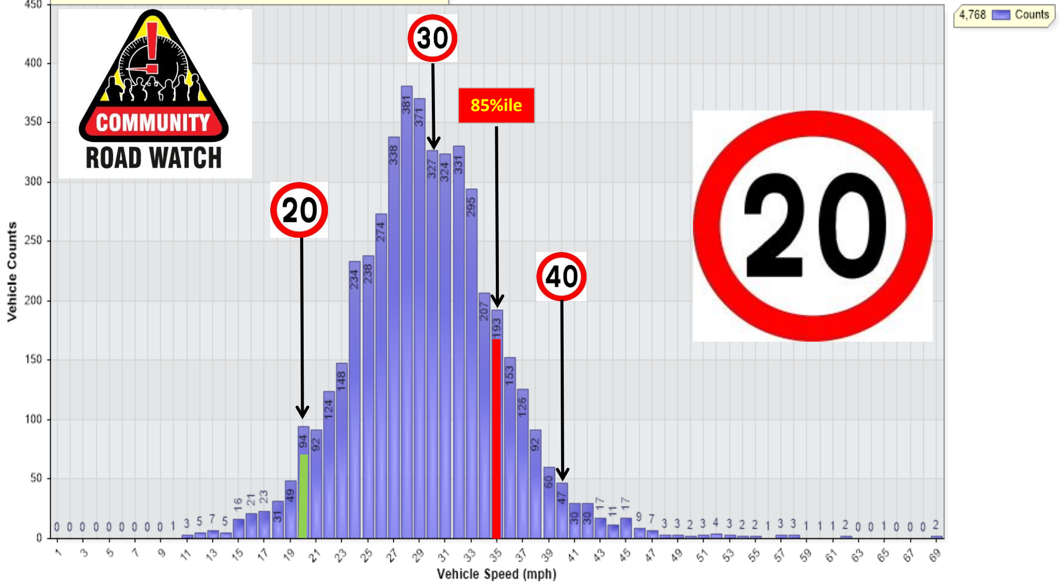
Vehicle Counts Vs. Speed [LogSOM-ChRd20-Dec24: Outgoing Direction]
