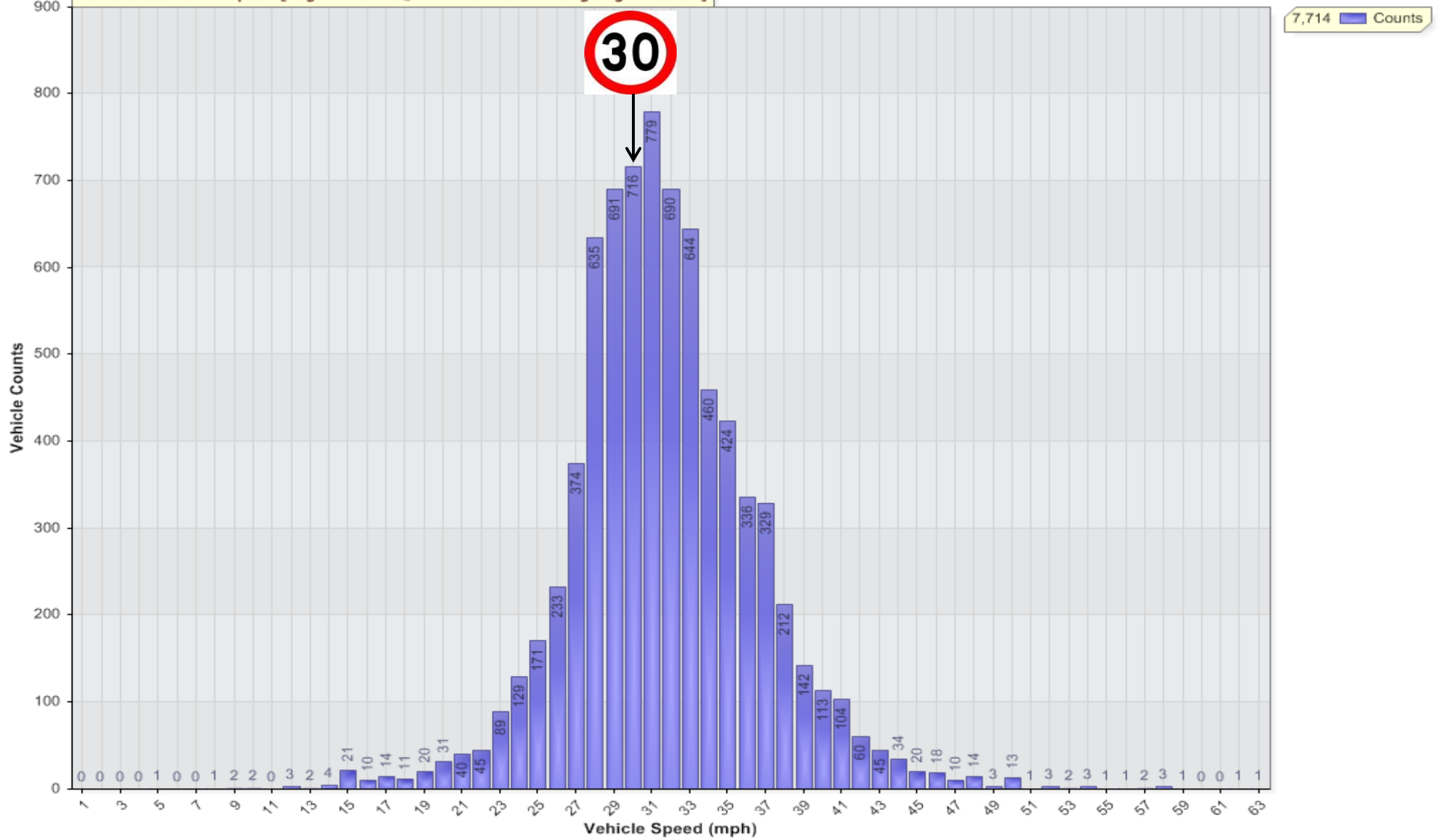
Vehicle Counts Vs. Speed [LogSOM-ChRd@BankAve-Nov21: Outgoing Direction]
