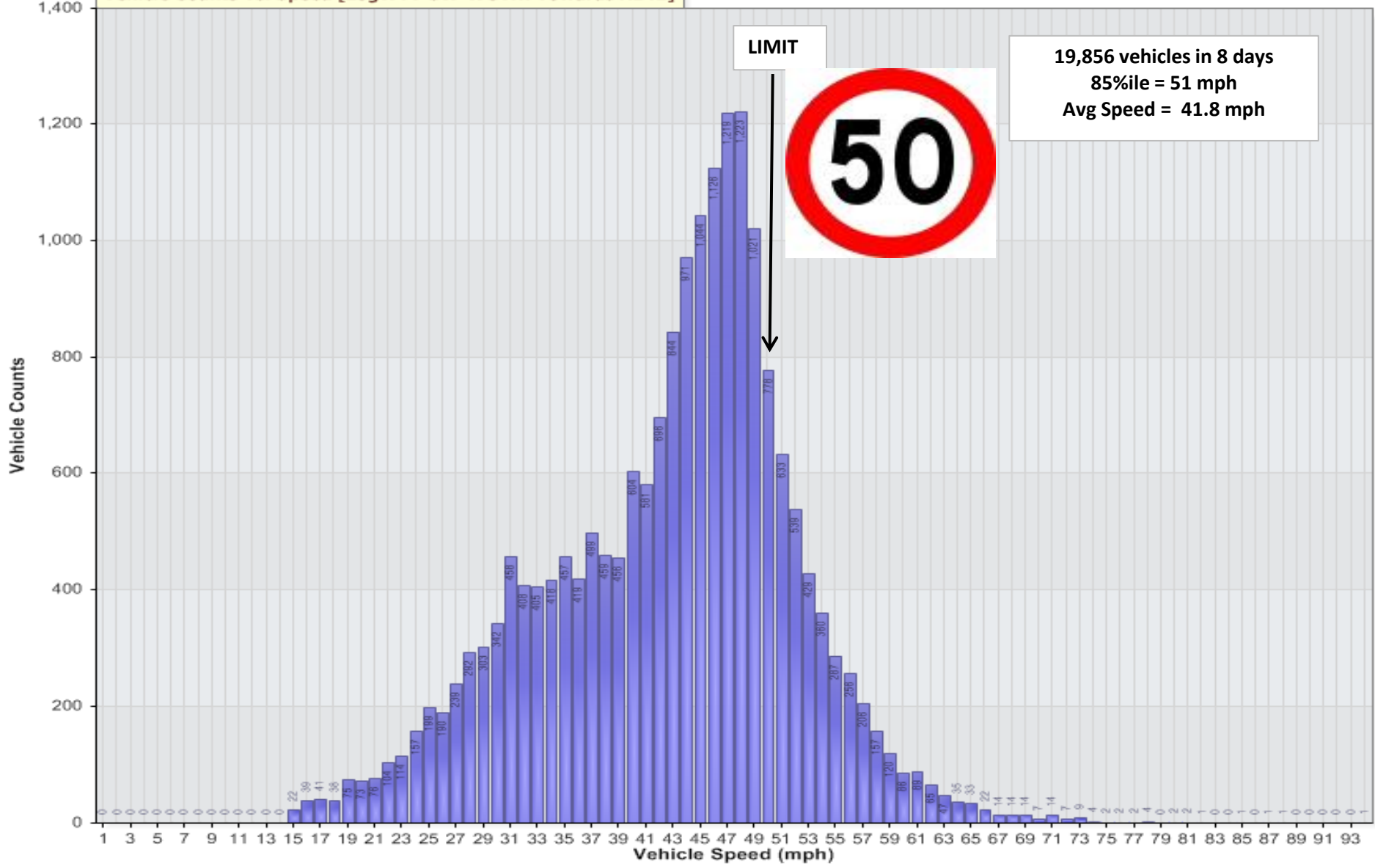
Vehicle Counts Vs. Speed [LogWYT-SW-WOTH: Towards A141]
