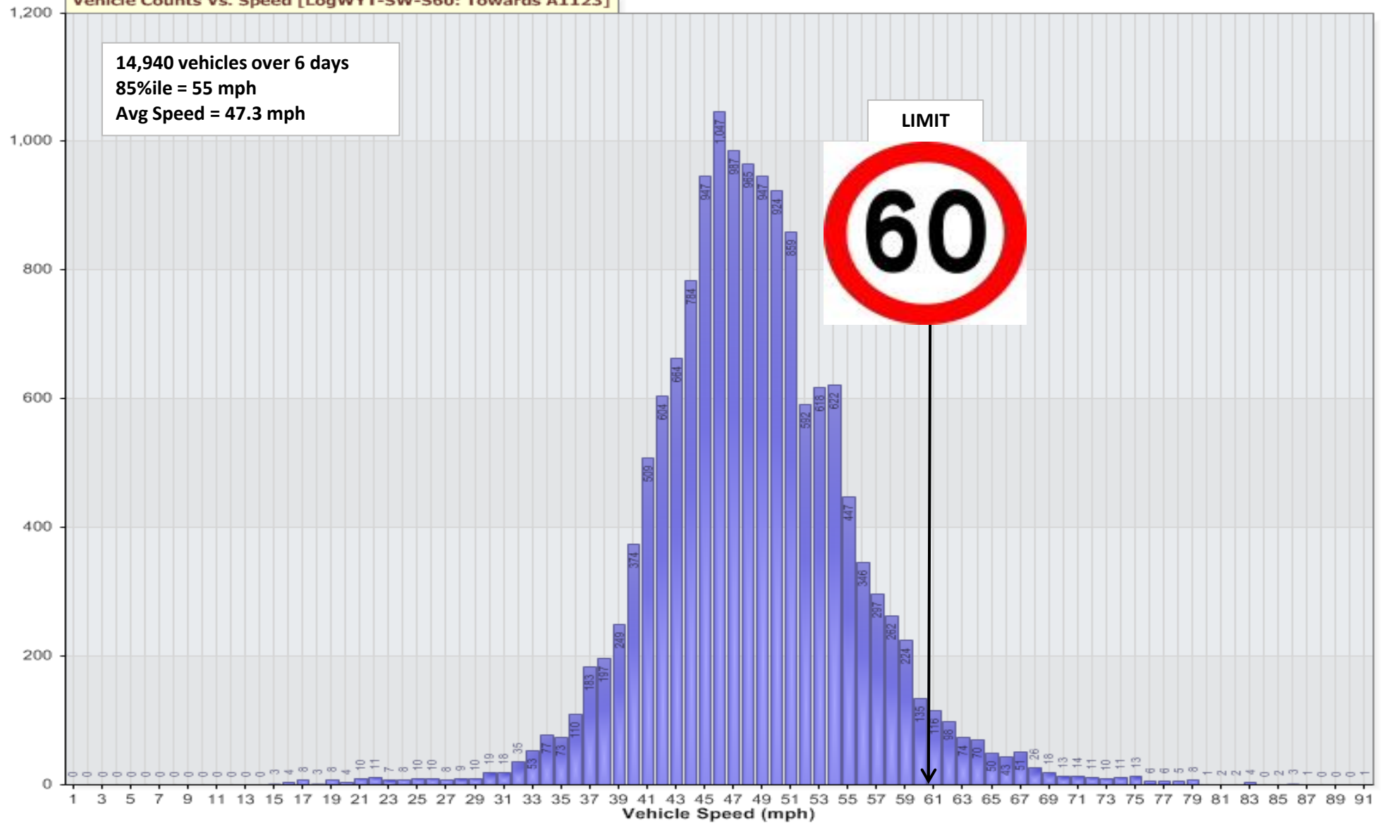
Vehicle Counts Vs. Speed [LogWYT-SW-S60: Towards A1123]
