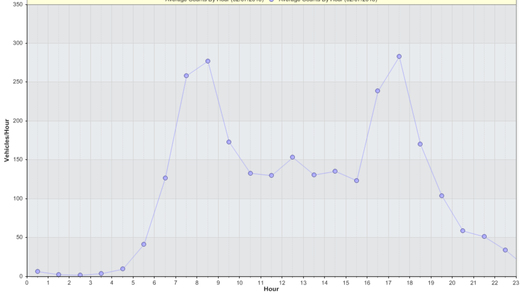
Towards A1123:Average Hourly Volume for Week of 02/07/2018 Average Counts By Hour (02/07/2018) —●— Average Counts By Hour (02/07/2018)
